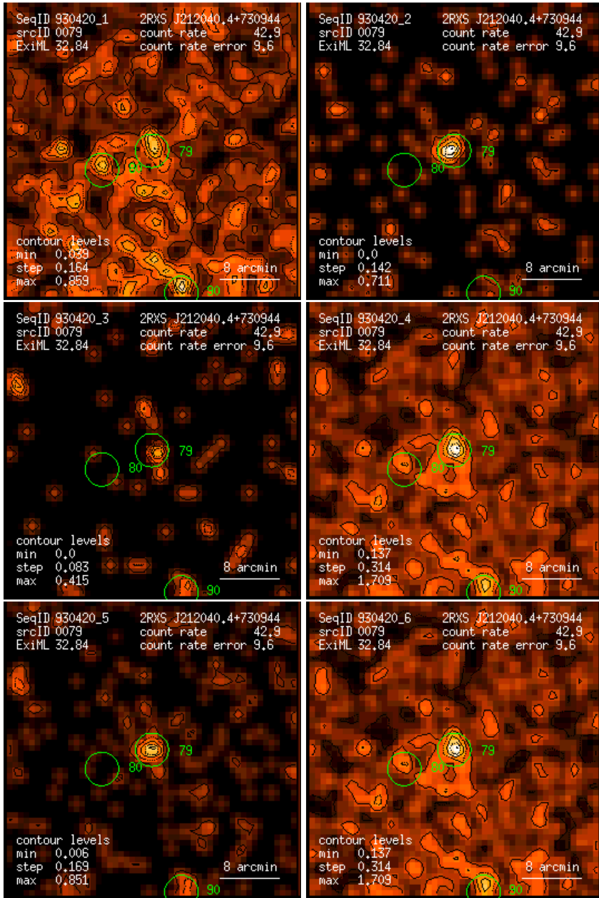
Figure 79: RASS 930420: detection 0079: band rate images, Gaussian filter: (1) PSPC channels 11 – 41, (2) 52 – 90, (3) 91 – 201, (4) 11 – 235, (5) 52 – 201, (6) 11 – 201. Broad band rates in counts/ks. Band rate contour levels in counts/ks/arcmin 2 .
