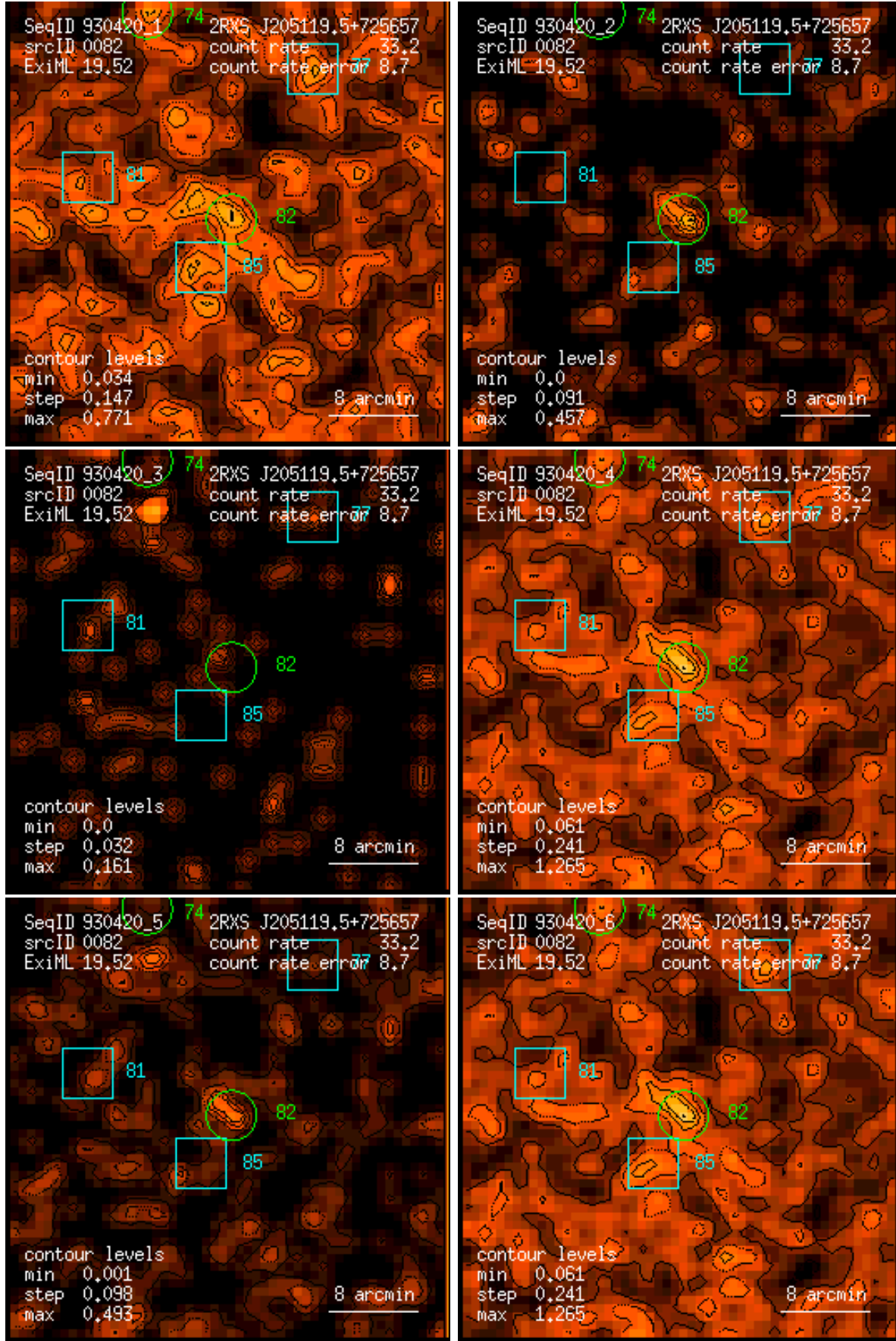
Figure 82: RASS 930420: detection 0082: band rate images, Gaussian filter: (1) PSPC channels 11 – 41, (2) 52 – 90, (3) 91 – 201, (4) 11 – 235, (5) 52 – 201, (6) 11 – 201. Broad band rates in counts/ks. Band rate contour levels in counts/ks/arcmin 2 .
