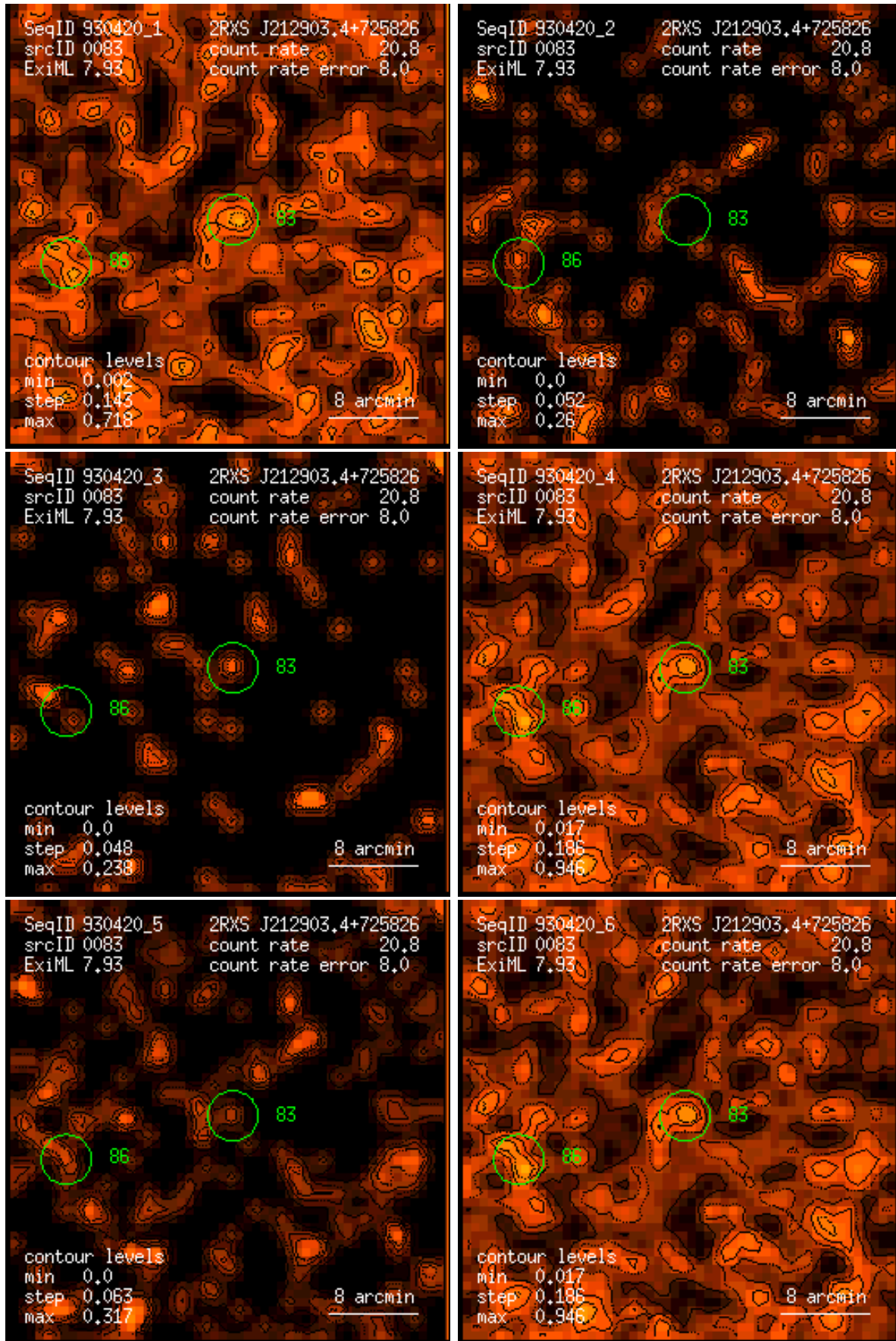
Figure 83: RASS 930420: detection 0083: band rate images, Gaussian filter: (1) PSPC channels 11 – 41, (2) 52 – 90, (3) 91 – 201, (4) 11 – 235, (5) 52 – 201, (6) 11 – 201. Broad band rates in counts/ks. Band rate contour levels in counts/ks/arcmin 2 .
