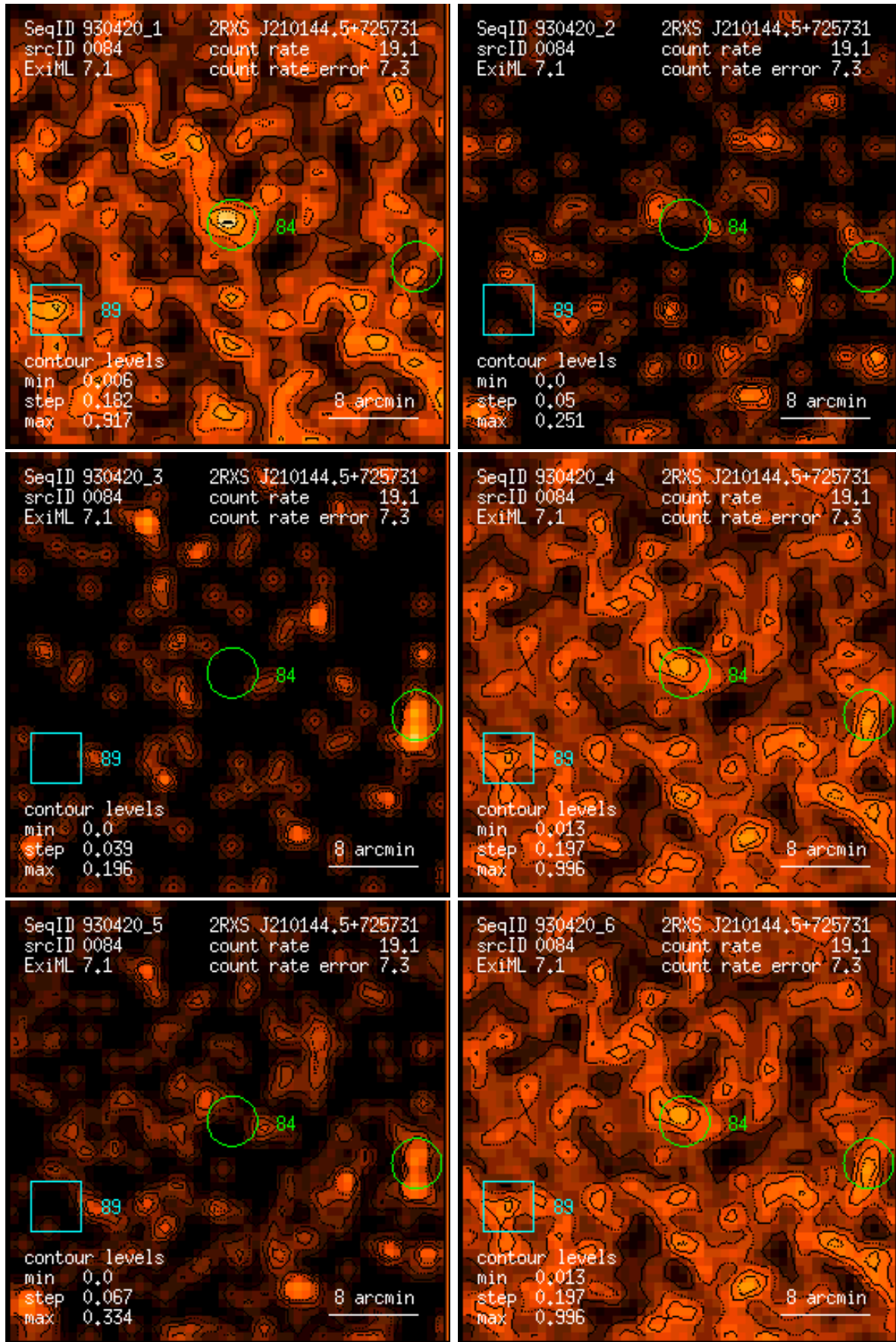
Figure 84: RASS 930420: detection 0084: band rate images, Gaussian filter: (1) PSPC channels 11 – 41, (2) 52 – 90, (3) 91 – 201, (4) 11 – 235, (5) 52 – 201, (6) 11 – 201. Broad band rates in counts/ks. Band rate contour levels in counts/ks/arcmin 2 .
