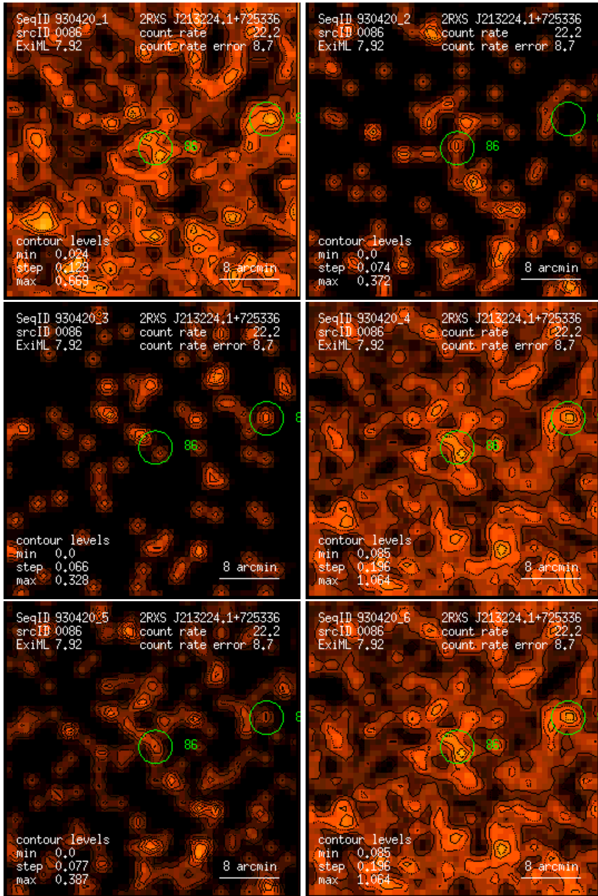
Figure 86: RASS 930420: detection 0086: band rate images, Gaussian filter: (1) PSPC channels 11 – 41, (2) 52 – 90, (3) 91 – 201, (4) 11 – 235, (5) 52 – 201, (6) 11 – 201. Broad band rates in counts/ks. Band rate contour levels in counts/ks/arcmin 2 .
