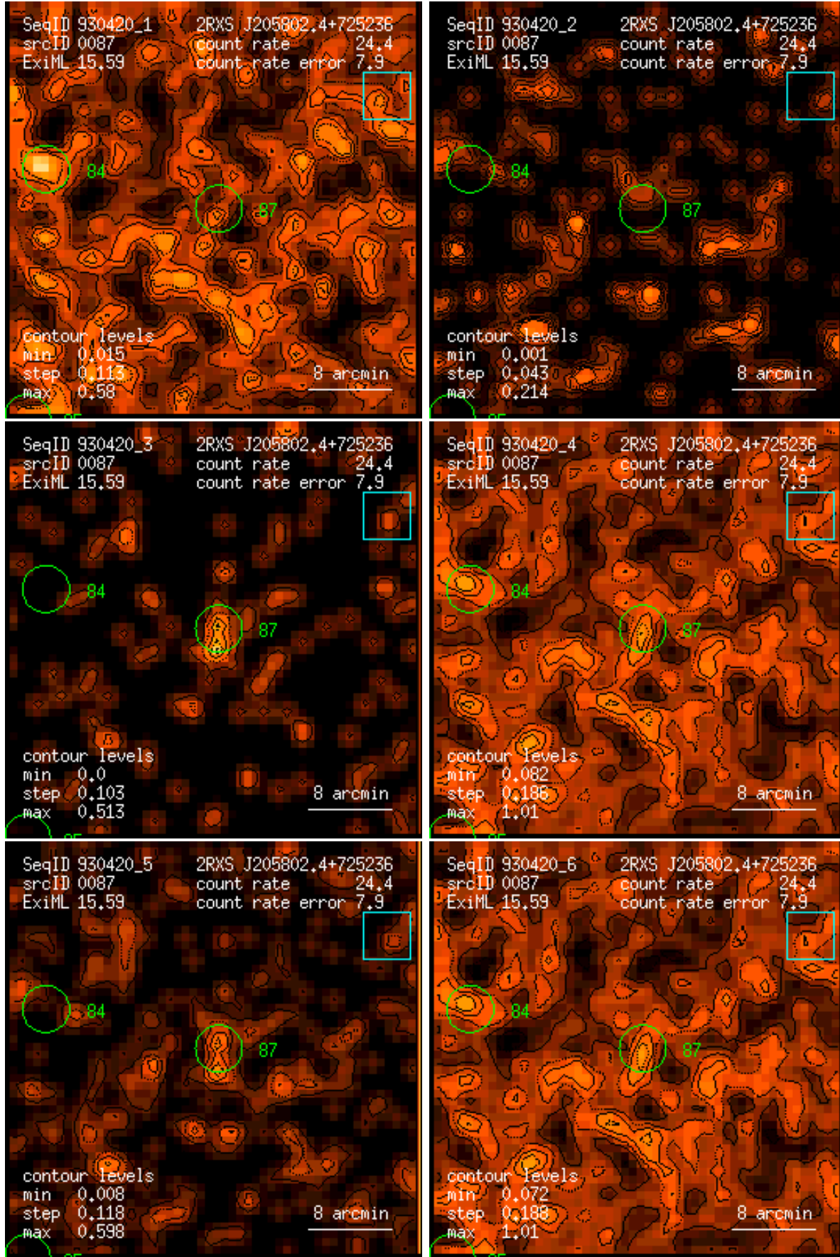
Figure 87: RASS 930420: detection 0087: band rate images, Gaussian filter: (1) PSPC channels 11 – 41, (2) 52 – 90, (3) 91 – 201, (4) 11 – 235, (5) 52 – 201, (6) 11 – 201. Broad band rates in counts/ks. Band rate contour levels in counts/ks/arcmin 2 .
