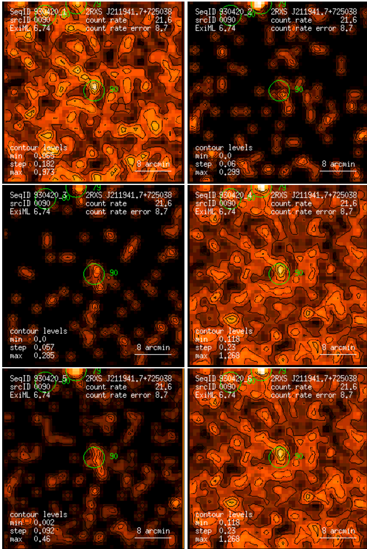
Figure 90: RASS 930420: detection 0090: band rate images, Gaussian filter: (1) PSPC channels 11 – 41, (2) 52 – 90, (3) 91 – 201, (4) 11 – 235, (5) 52 – 201, (6) 11 – 201. Broad band rates in counts/ks. Band rate contour levels in counts/ks/arcmin 2 .
