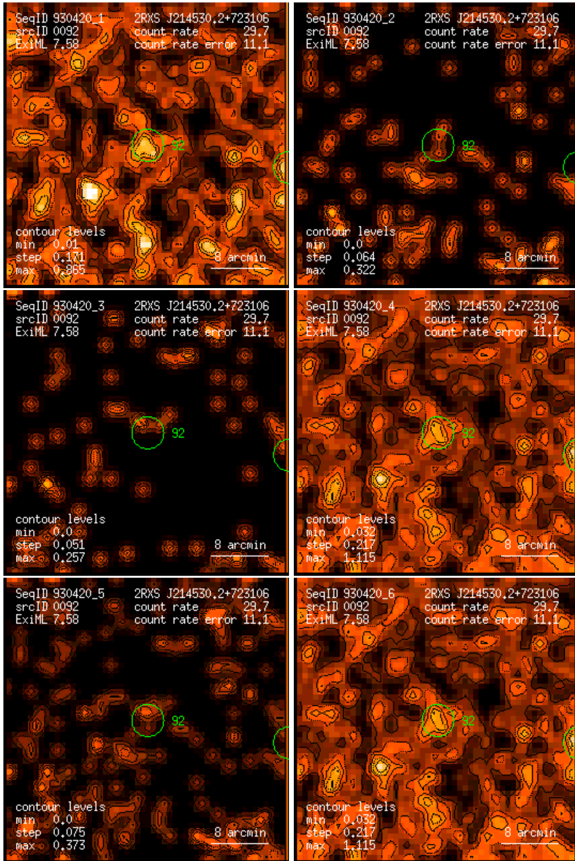
Figure 92: RASS 930420: detection 0092: band rate images, Gaussian filter: (1) PSPC channels 11 – 41, (2) 52 – 90, (3) 91 – 201, (4) 11 – 235, (5) 52 – 201, (6) 11 – 201. Broad band rates in counts/ks. Band rate contour levels in counts/ks/arcmin 2 .
