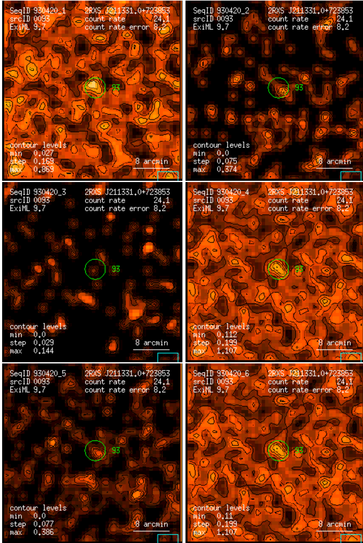
Figure 93: RASS 930420: detection 0093: band rate images, Gaussian filter: (1) PSPC channels 11 – 41, (2) 52 – 90, (3) 91 – 201, (4) 11 – 235, (5) 52 – 201, (6) 11 – 201. Broad band rates in counts/ks. Band rate contour levels in counts/ks/arcmin 2 .
