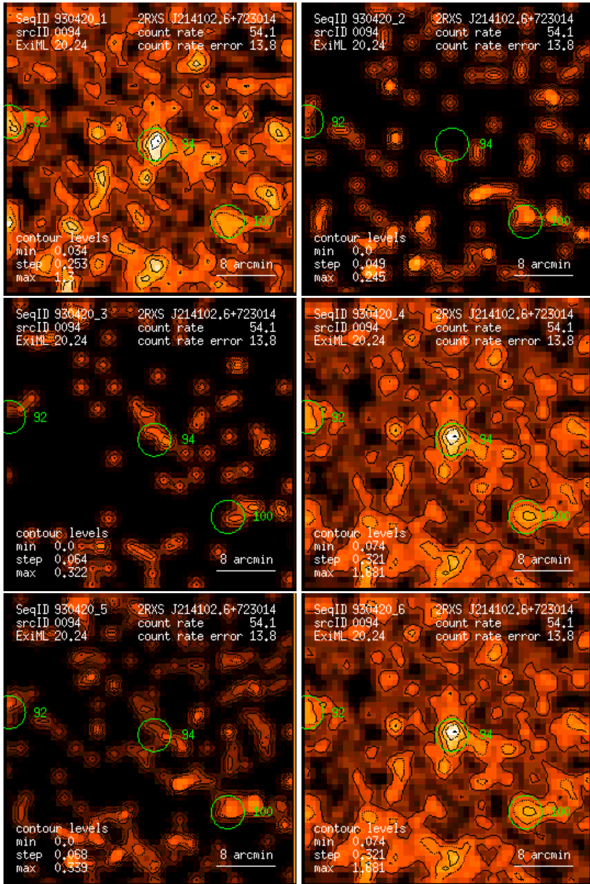
Figure 94: RASS 930420: detection 0094: band rate images, Gaussian filter: (1) PSPC channels 11 – 41, (2) 52 – 90, (3) 91 – 201, (4) 11 – 235, (5) 52 – 201, (6) 11 – 201. Broad band rates in counts/ks. Band rate contour levels in counts/ks/arcmin 2 .
