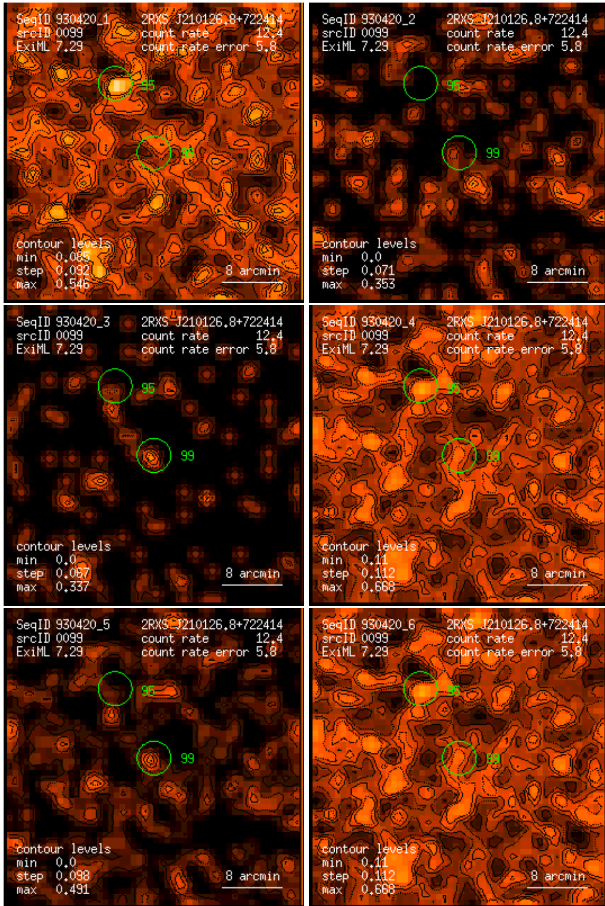
Figure 99: RASS 930420: detection 0099: band rate images, Gaussian filter: (1) PSPC channels 11 – 41, (2) 52 – 90, (3) 91 – 201, (4) 11 – 235, (5) 52 – 201, (6) 11 – 201. Broad band rates in counts/ks. Band rate contour levels in counts/ks/arcmin 2 .
