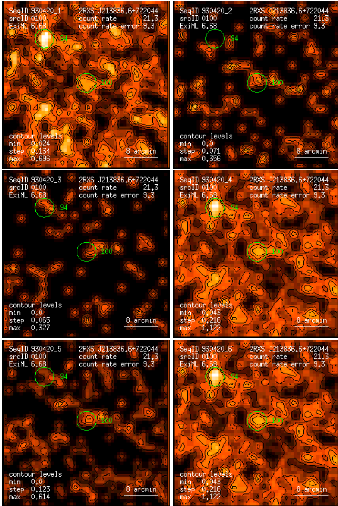
Figure 100: RASS 930420: detection 0100: band rate images, Gaussian filter: (1) PSPC channels 11 – 41, (2) 52 – 90, (3) 91 – 201, (4) 11 – 235, (5) 52 – 201, (6) 11 – 201. Broad band rates in counts/ks. Band rate contour levels in counts/ks/arcmin 2 .
