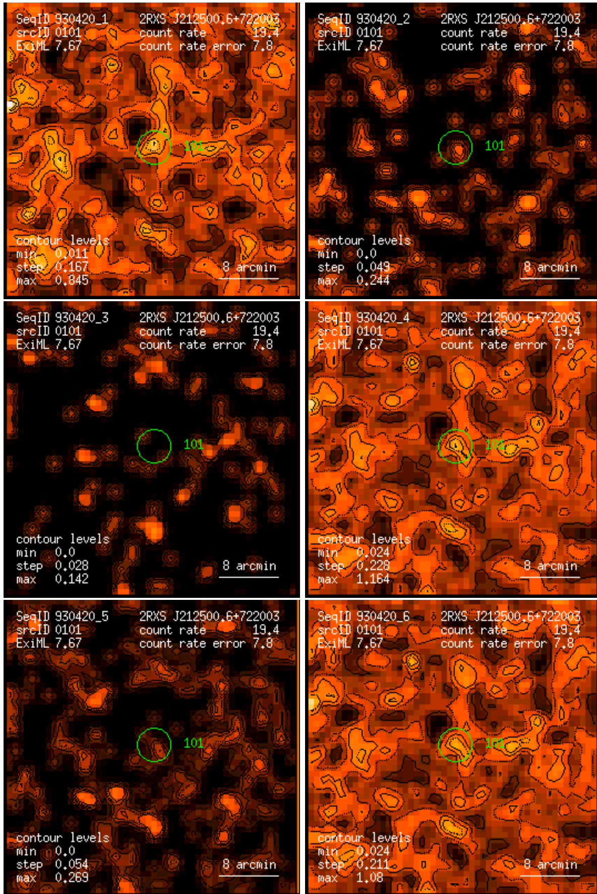
Figure 101: RASS 930420: detection 0101: band rate images, Gaussian filter: (1) PSPC channels 11 – 41, (2) 52 – 90, (3) 91 – 201, (4) 11 – 235, (5) 52 – 201, (6) 11 – 201. Broad band rates in counts/ks. Band rate contour levels in counts/ks/arcmin 2 .
