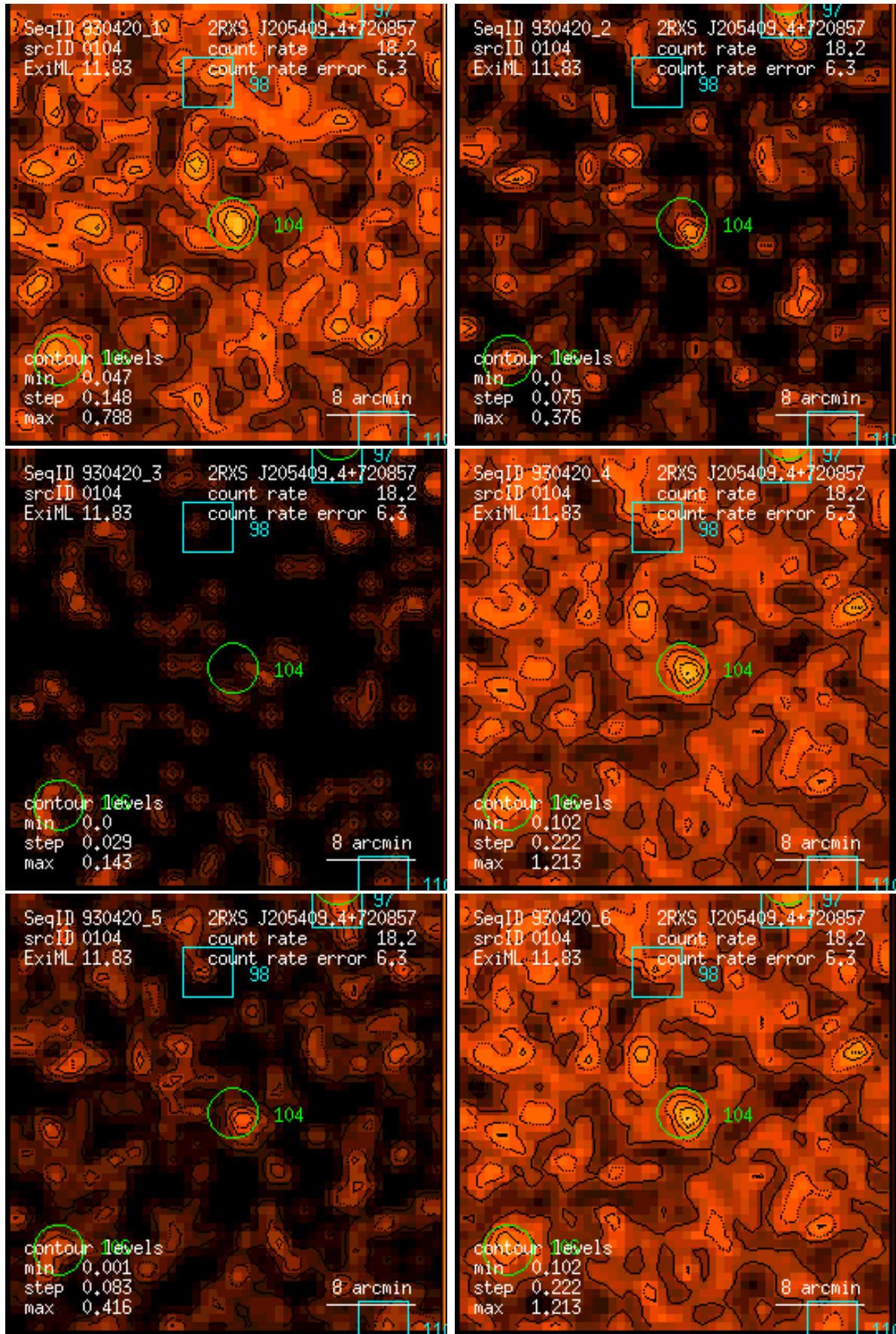
Figure 104: RASS 930420: detection 0104: band rate images, Gaussian filter: (1) PSPC channels 11 – 41, (2) 52 – 90, (3) 91 – 201, (4) 11 – 235, (5) 52 – 201, (6) 11 – 201. Broad band rates in counts/ks. Band rate contour levels in counts/ks/arcmin 2 .
