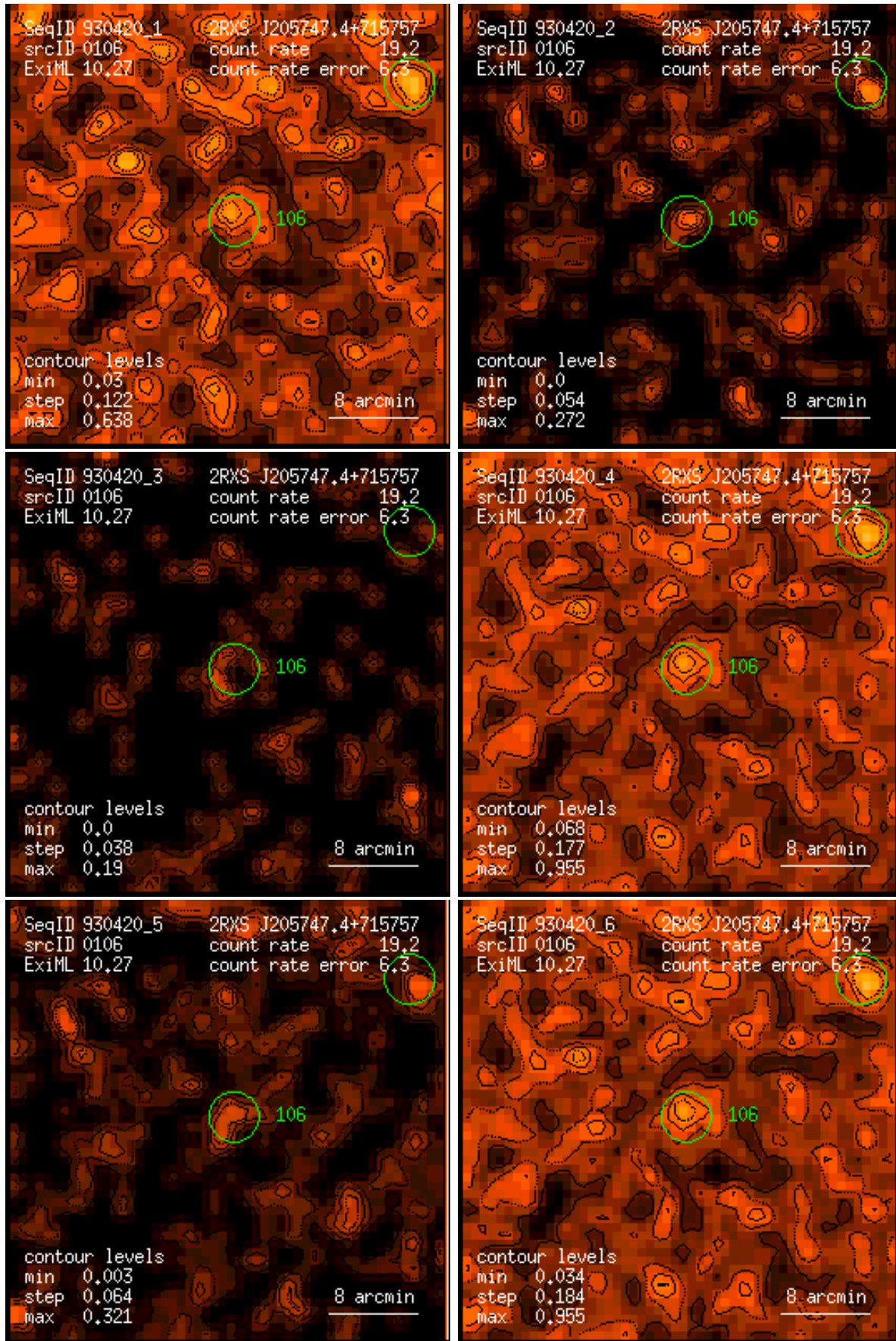
Figure 106: RASS 930420: detection 0106: band rate images, Gaussian filter: (1) PSPC channels 11 – 41, (2) 52 – 90, (3) 91 – 201, (4) 11 – 235, (5) 52 – 201, (6) 11 – 201. Broad band rates in counts/ks. Band rate contour levels in counts/ks/arcmin 2 .
