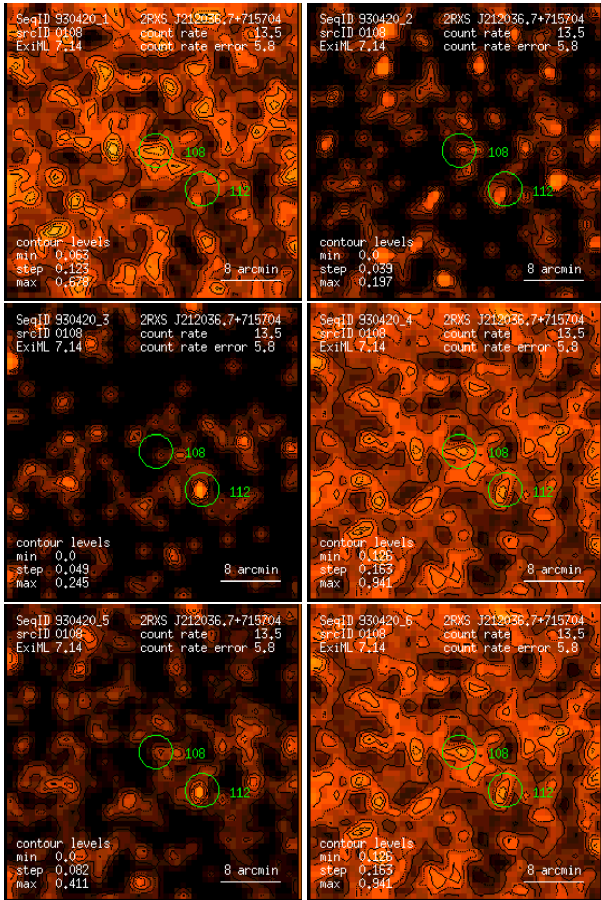
Figure 108: RASS 930420: detection 0108: band rate images, Gaussian filter: (1) PSPC channels 11 – 41, (2) 52 – 90, (3) 91 – 201, (4) 11 – 235, (5) 52 – 201, (6) 11 – 201. Broad band rates in counts/ks. Band rate contour levels in counts/ks/arcmin 2 .
