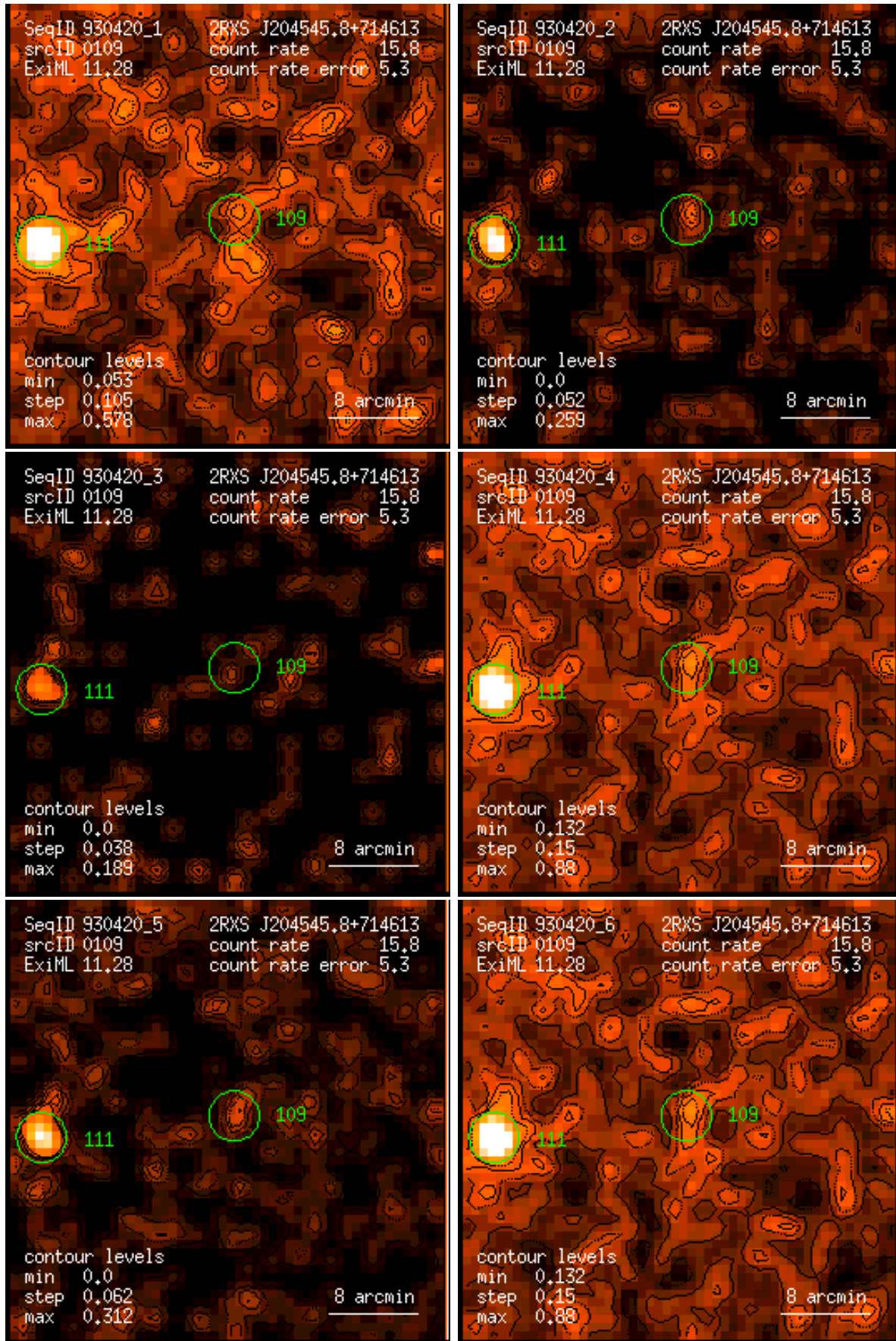
Figure 109: RASS 930420: detection 0109: band rate images, Gaussian filter: (1) PSPC channels 11 – 41, (2) 52 – 90, (3) 91 – 201, (4) 11 – 235, (5) 52 – 201, (6) 11 – 201. Broad band rates in counts/ks. Band rate contour levels in counts/ks/arcmin 2 .
