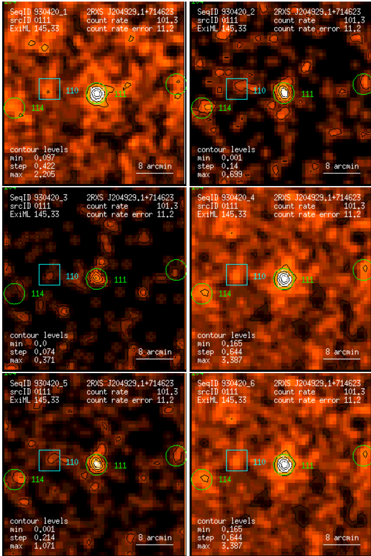
Figure 111: RASS 930420: detection 0111: band rate images, Gaussian filter: (1) PSPC channels 11 – 41, (2) 52 – 90, (3) 91 – 201, (4) 11 – 235, (5) 52 – 201, (6) 11 – 201. Broad band rates in counts/ks. Band rate contour levels in counts/ks/arcmin 2 .
