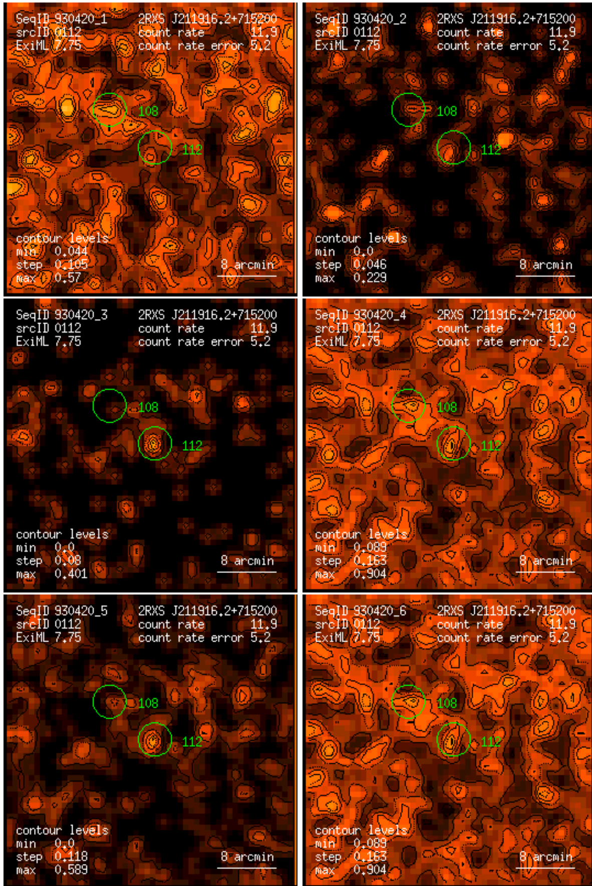
Figure 112: RASS 930420: detection 0112: band rate images, Gaussian filter: (1) PSPC channels 11 – 41, (2) 52 – 90, (3) 91 – 201, (4) 11 – 235, (5) 52 – 201, (6) 11 – 201. Broad band rates in counts/ks. Band rate contour levels in counts/ks/arcmin 2 .
