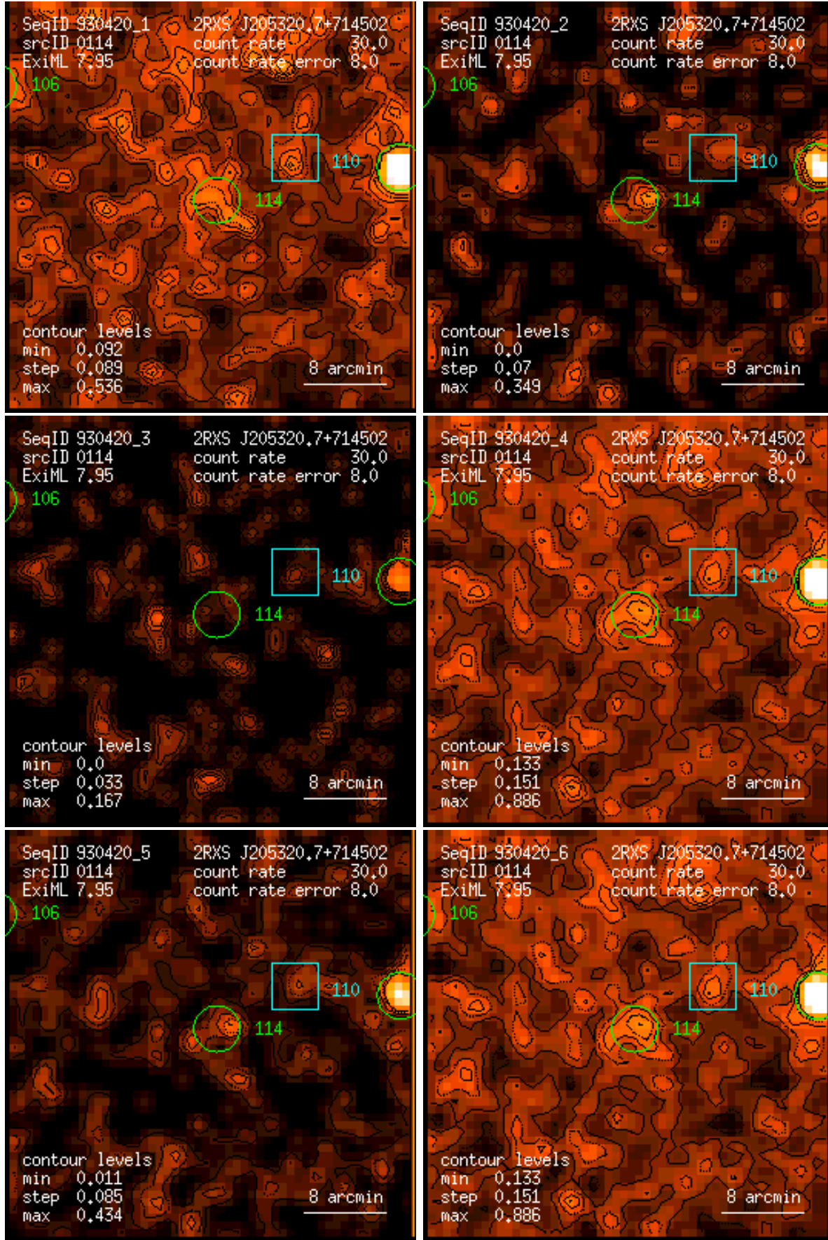
Figure 114: RASS 930420: detection 0114: band rate images, Gaussian filter: (1) PSPC channels 11 – 41, (2) 52 – 90, (3) 91 – 201, (4) 11 – 235, (5) 52 – 201, (6) 11 – 201. Broad band rates in counts/ks. Band rate contour levels in counts/ks/arcmin 2 .
