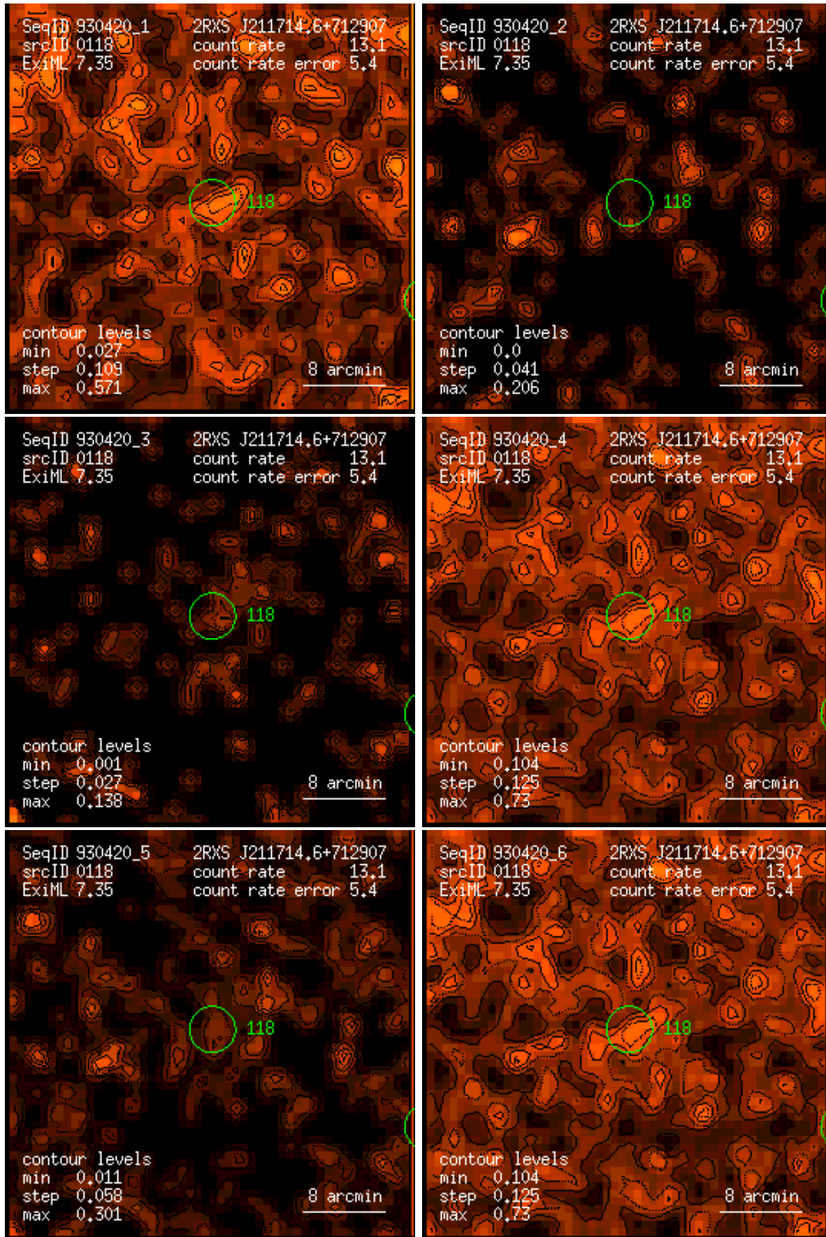
Figure 118: RASS 930420: detection 0118: band rate images, Gaussian filter: (1) PSPC channels 11 – 41, (2) 52 – 90, (3) 91 – 201, (4) 11 – 235, (5) 52 – 201, (6) 11 – 201. Broad band rates in counts/ks. Band rate contour levels in counts/ks/arcmin 2 .
