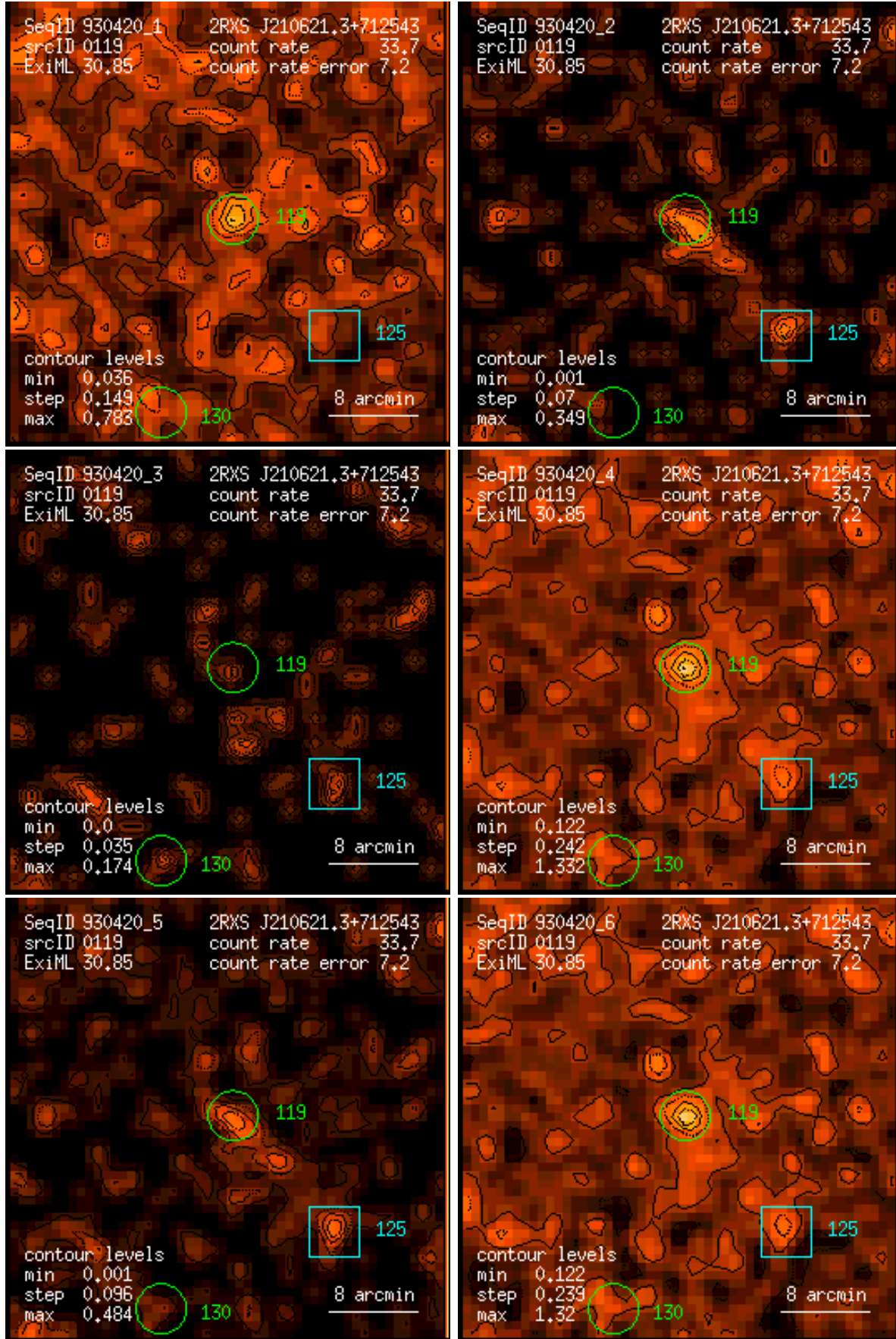
Figure 119: RASS 930420: detection 0119: band rate images, Gaussian filter: (1) PSPC channels 11 – 41, (2) 52 – 90, (3) 91 – 201, (4) 11 – 235, (5) 52 – 201, (6) 11 – 201. Broad band rates in counts/ks. Band rate contour levels in counts/ks/arcmin 2 .
