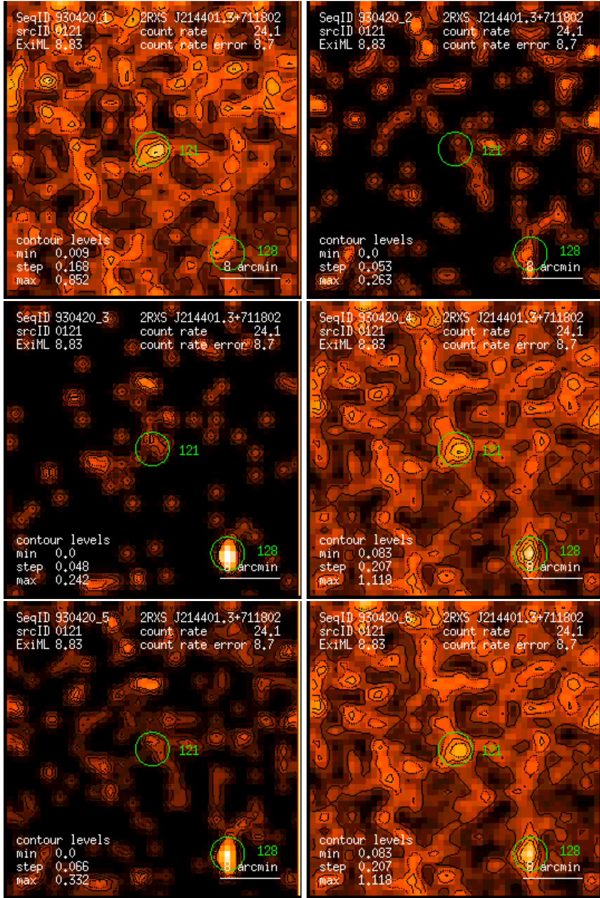
Figure 121: RASS 930420: detection 0121: band rate images, Gaussian filter: (1) PSPC channels 11 – 41, (2) 52 – 90, (3) 91 – 201, (4) 11 – 235, (5) 52 – 201, (6) 11 – 201. Broad band rates in counts/ks. Band rate contour levels in counts/ks/arcmin 2 .
