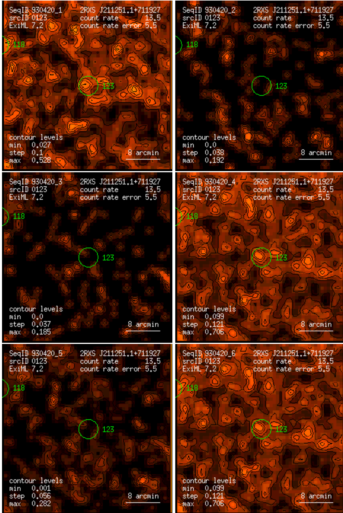
Figure 123: RASS 930420: detection 0123: band rate images, Gaussian filter: (1) PSPC channels 11 – 41, (2) 52 – 90, (3) 91 – 201, (4) 11 – 235, (5) 52 – 201, (6) 11 – 201. Broad band rates in counts/ks. Band rate contour levels in counts/ks/arcmin 2 .
