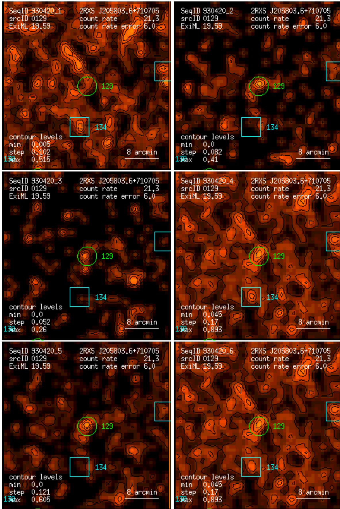
Figure 129: RASS 930420: detection 0129: band rate images, Gaussian filter: (1) PSPC channels 11 – 41, (2) 52 – 90, (3) 91 – 201, (4) 11 – 235, (5) 52 – 201, (6) 11 – 201. Broad band rates in counts/ks. Band rate contour levels in counts/ks/arcmin 2 .
