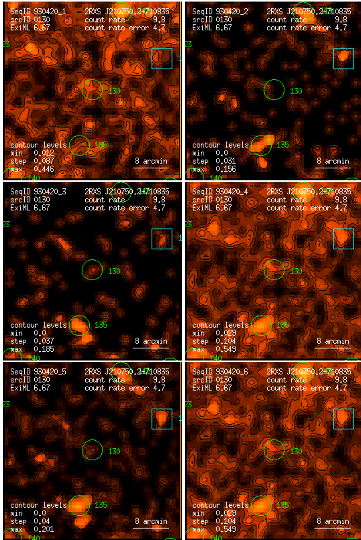
Figure 130: RASS 930420: detection 0130: band rate images, Gaussian filter: (1) PSPC channels 11 – 41, (2) 52 – 90, (3) 91 – 201, (4) 11 – 235, (5) 52 – 201, (6) 11 – 201. Broad band rates in counts/ks. Band rate contour levels in counts/ks/arcmin 2 .
