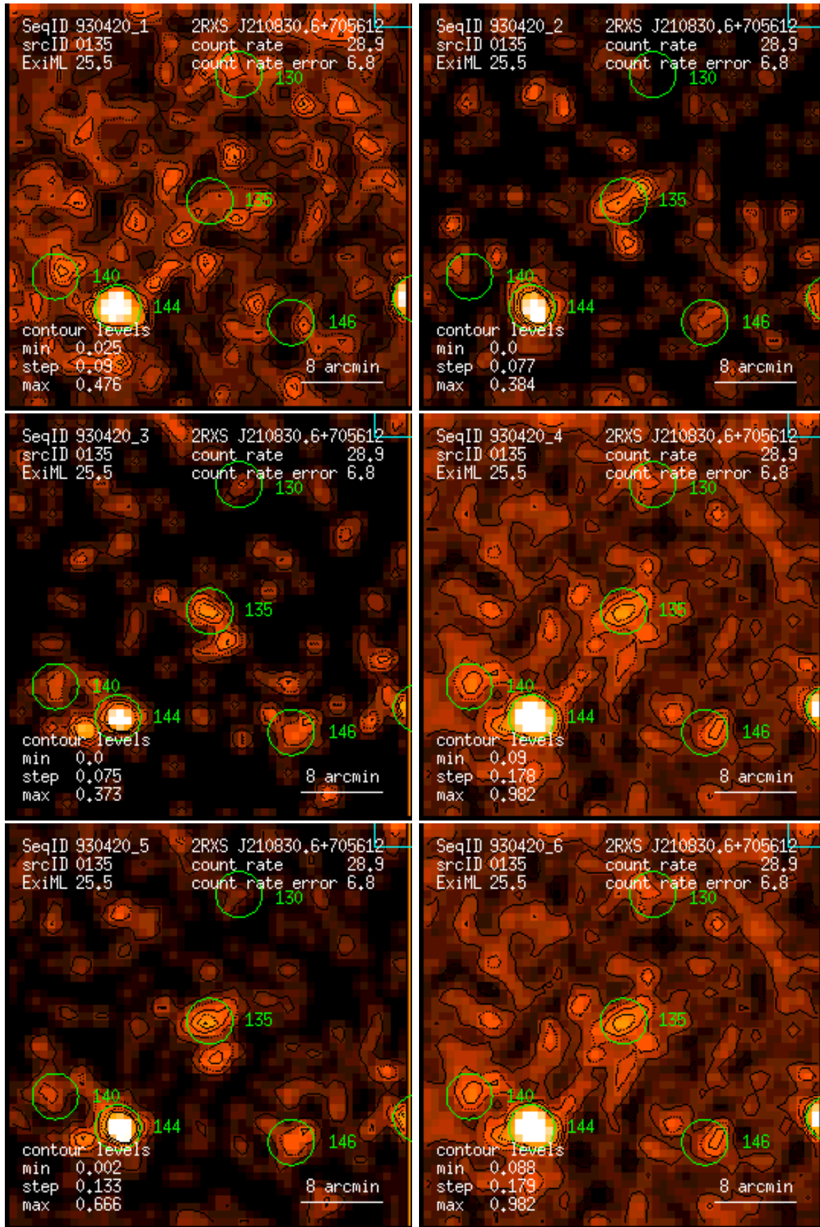
Figure 135: RASS 930420: detection 0135: band rate images, Gaussian filter: (1) PSPC channels 11 – 41, (2) 52 – 90, (3) 91 – 201, (4) 11 – 235, (5) 52 – 201, (6) 11 – 201. Broad band rates in counts/ks. Band rate contour levels in counts/ks/arcmin 2 .
