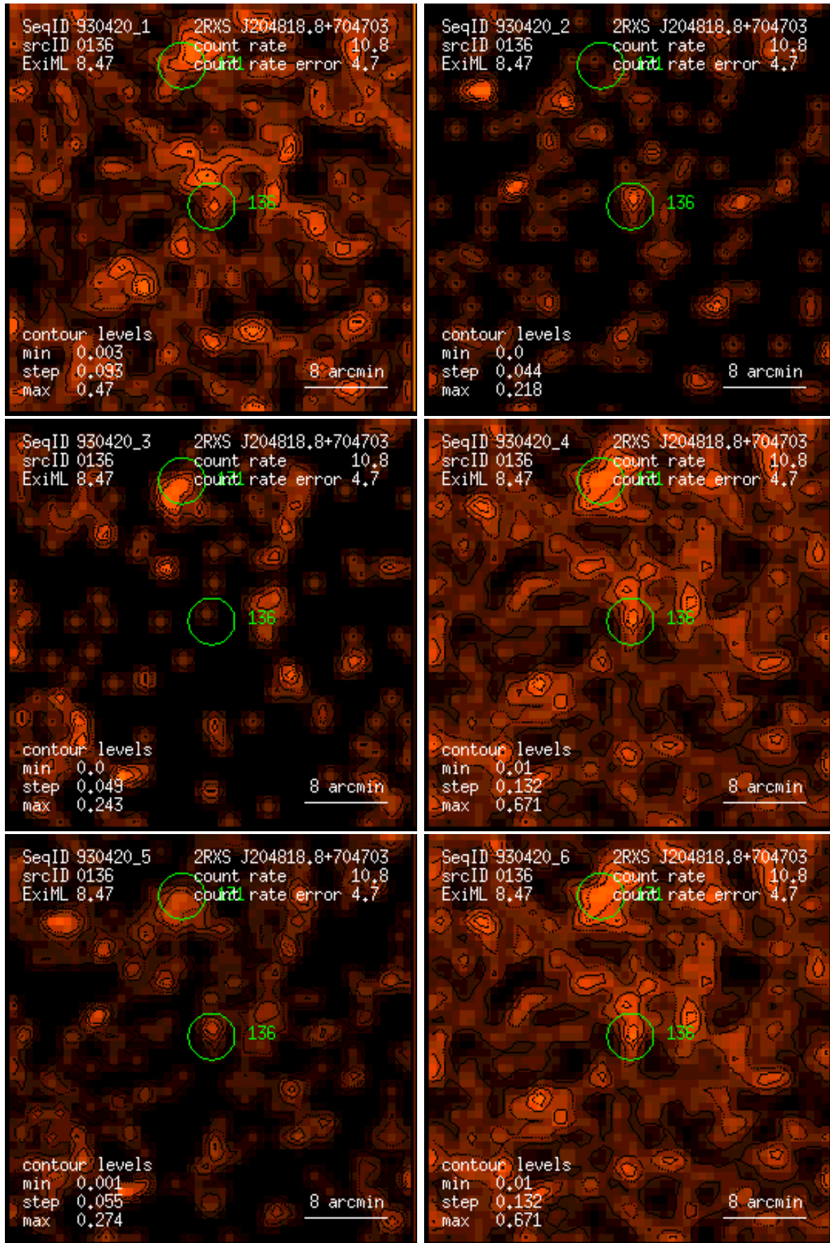
Figure 136: RASS 930420: detection 0136: band rate images, Gaussian filter: (1) PSPC channels 11 – 41, (2) 52 – 90, (3) 91 – 201, (4) 11 – 235, (5) 52 – 201, (6) 11 – 201. Broad band rates in counts/ks. Band rate contour levels in counts/ks/arcmin 2 .
