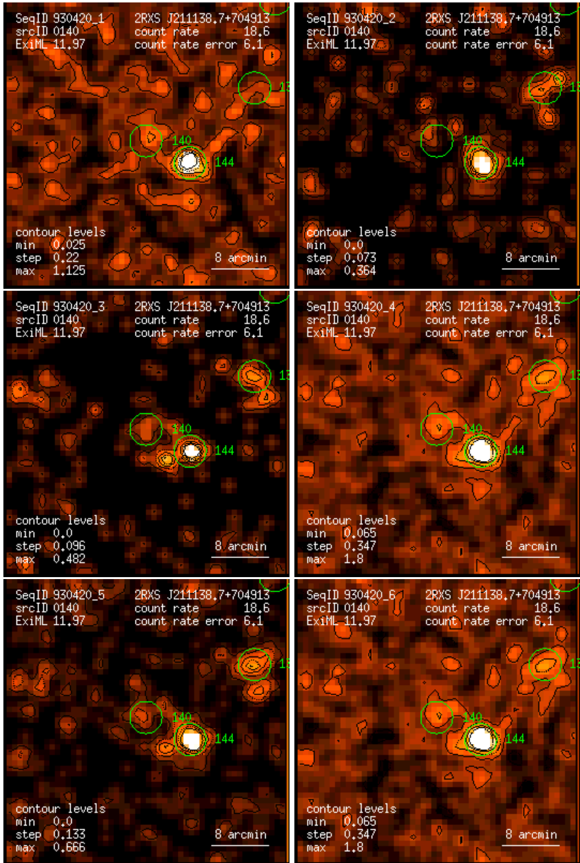
Figure 140: RASS 930420: detection 0140: band rate images, Gaussian filter: (1) PSPC channels 11 – 41, (2) 52 – 90, (3) 91 – 201, (4) 11 – 235, (5) 52 – 201, (6) 11 – 201. Broad band rates in counts/ks. Band rate contour levels in counts/ks/arcmin 2 .
