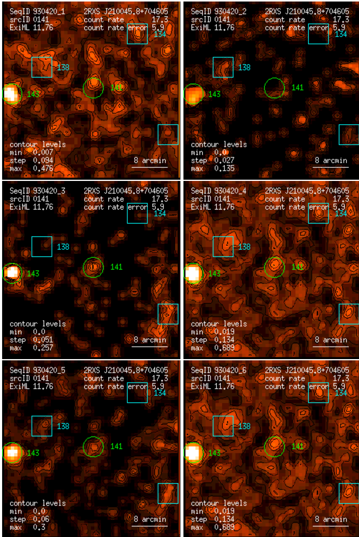
Figure 141: RASS 930420: detection 0141: band rate images, Gaussian filter: (1) PSPC channels 11 – 41, (2) 52 – 90, (3) 91 – 201, (4) 11 – 235, (5) 52 – 201, (6) 11 – 201. Broad band rates in counts/ks. Band rate contour levels in counts/ks/arcmin 2 .
