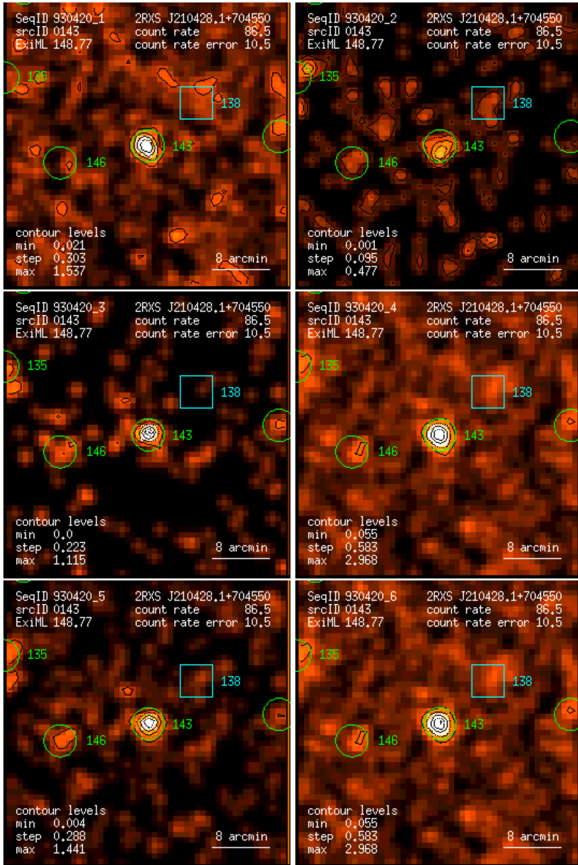
Figure 143: RASS 930420: detection 0143: band rate images, Gaussian filter: (1) PSPC channels 11 – 41, (2) 52 – 90, (3) 91 – 201, (4) 11 – 235, (5) 52 – 201, (6) 11 – 201. Broad band rates in counts/ks. Band rate contour levels in counts/ks/arcmin 2 .
