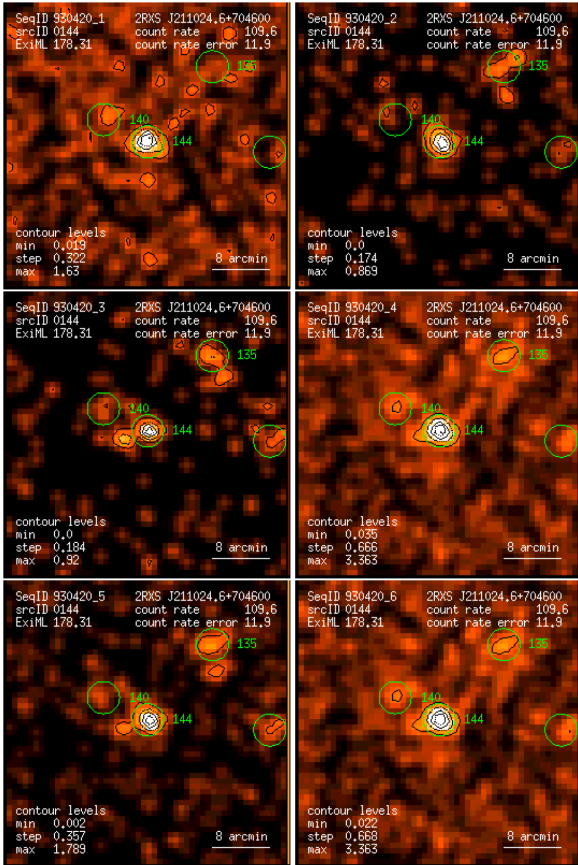
Figure 144: RASS 930420: detection 0144: band rate images, Gaussian filter: (1) PSPC channels 11 – 41, (2) 52 – 90, (3) 91 – 201, (4) 11 – 235, (5) 52 – 201, (6) 11 – 201. Broad band rates in counts/ks. Band rate contour levels in counts/ks/arcmin 2 .
