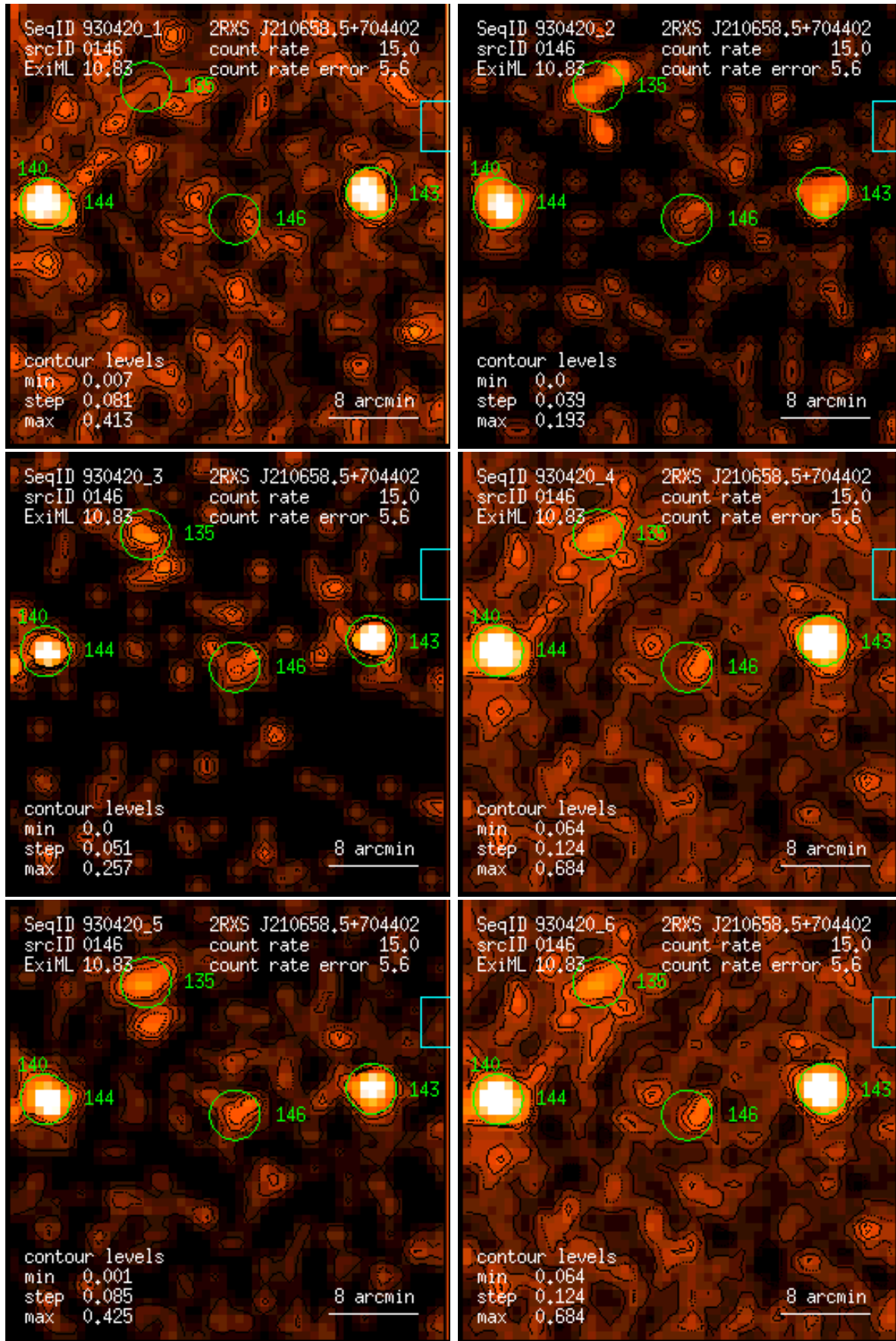
Figure 146: RASS 930420: detection 0146: band rate images, Gaussian filter: (1) PSPC channels 11 – 41, (2) 52 – 90, (3) 91 – 201, (4) 11 – 235, (5) 52 – 201, (6) 11 – 201. Broad band rates in counts/ks. Band rate contour levels in counts/ks/arcmin 2 .
