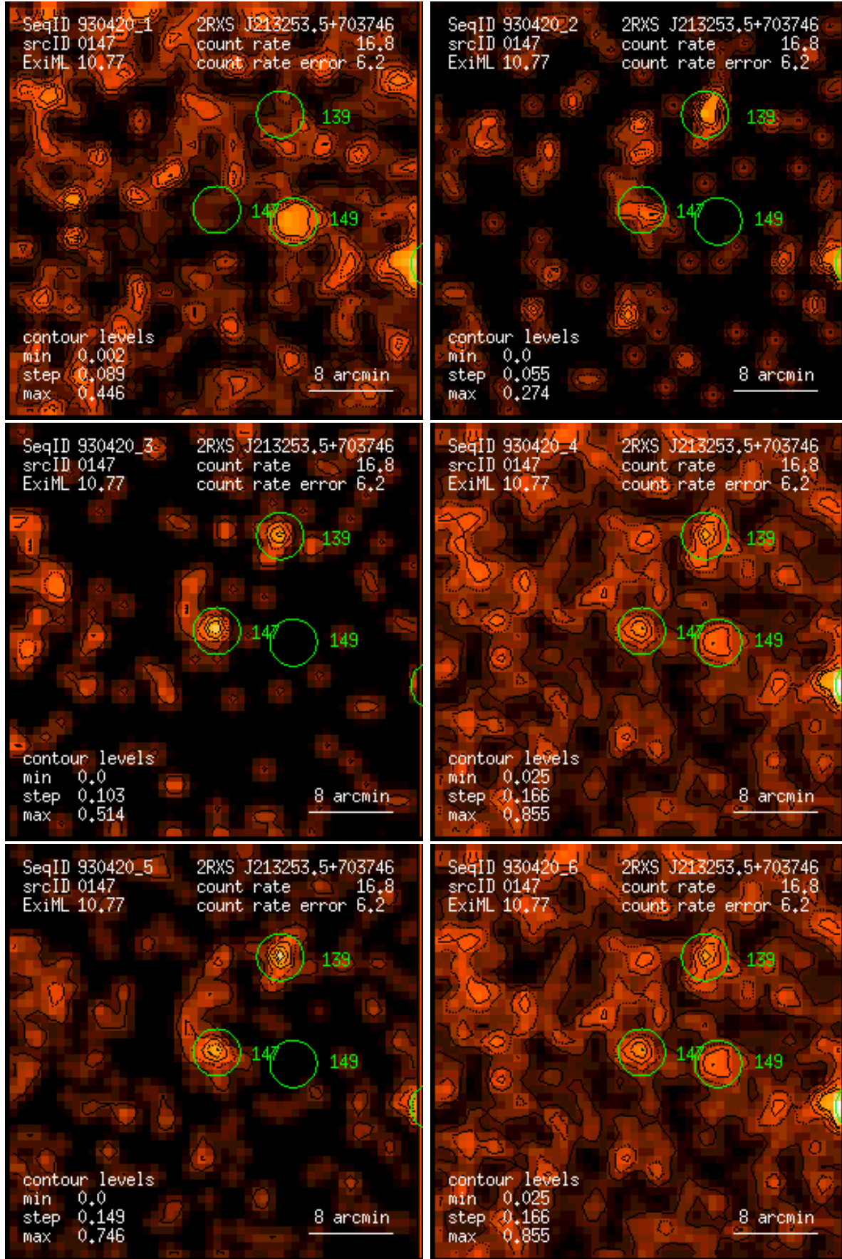
Figure 147: RASS 930420: detection 0147: band rate images, Gaussian filter: (1) PSPC channels 11 – 41, (2) 52 – 90, (3) 91 – 201, (4) 11 – 235, (5) 52 – 201, (6) 11 – 201. Broad band rates in counts/ks. Band rate contour levels in counts/ks/arcmin 2 .
