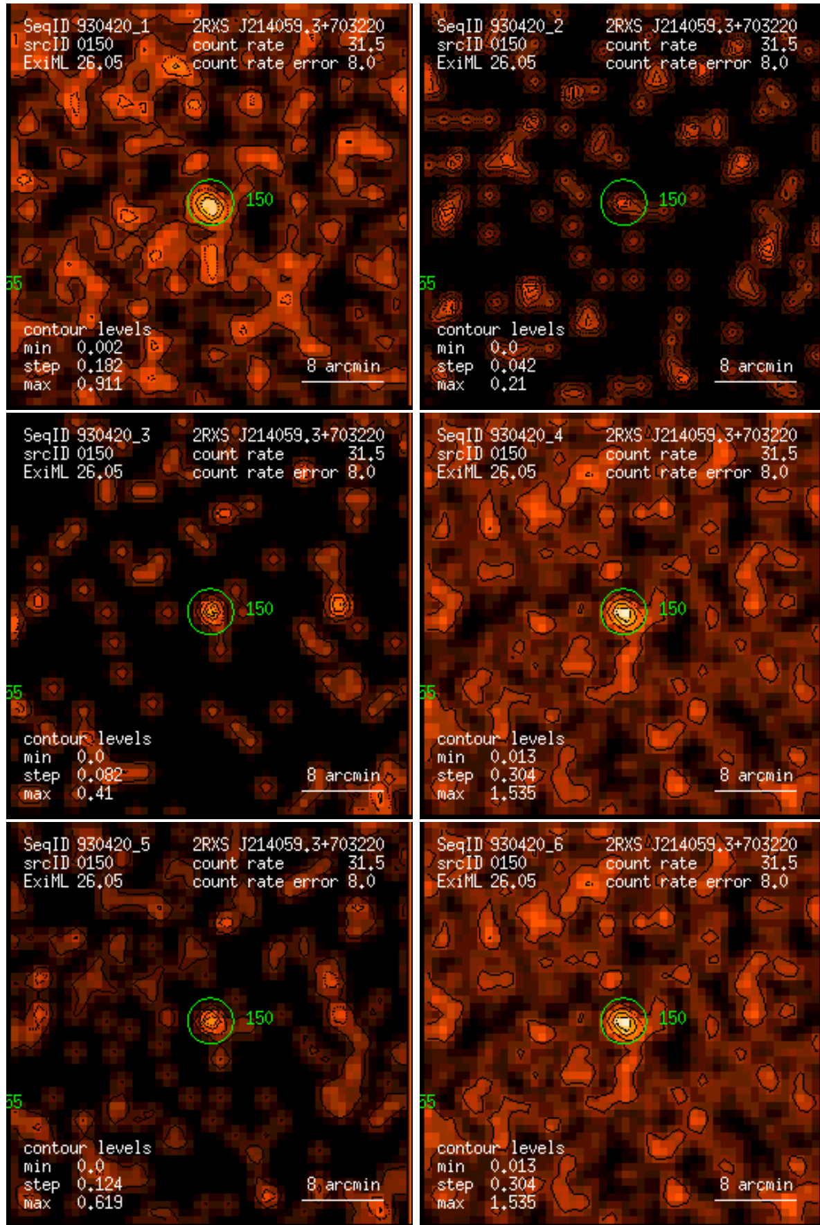
Figure 150: RASS 930420: detection 0150: band rate images, Gaussian filter: (1) PSPC channels 11 – 41, (2) 52 – 90, (3) 91 – 201, (4) 11 – 235, (5) 52 – 201, (6) 11 – 201. Broad band rates in counts/ks. Band rate contour levels in counts/ks/arcmin 2 .
