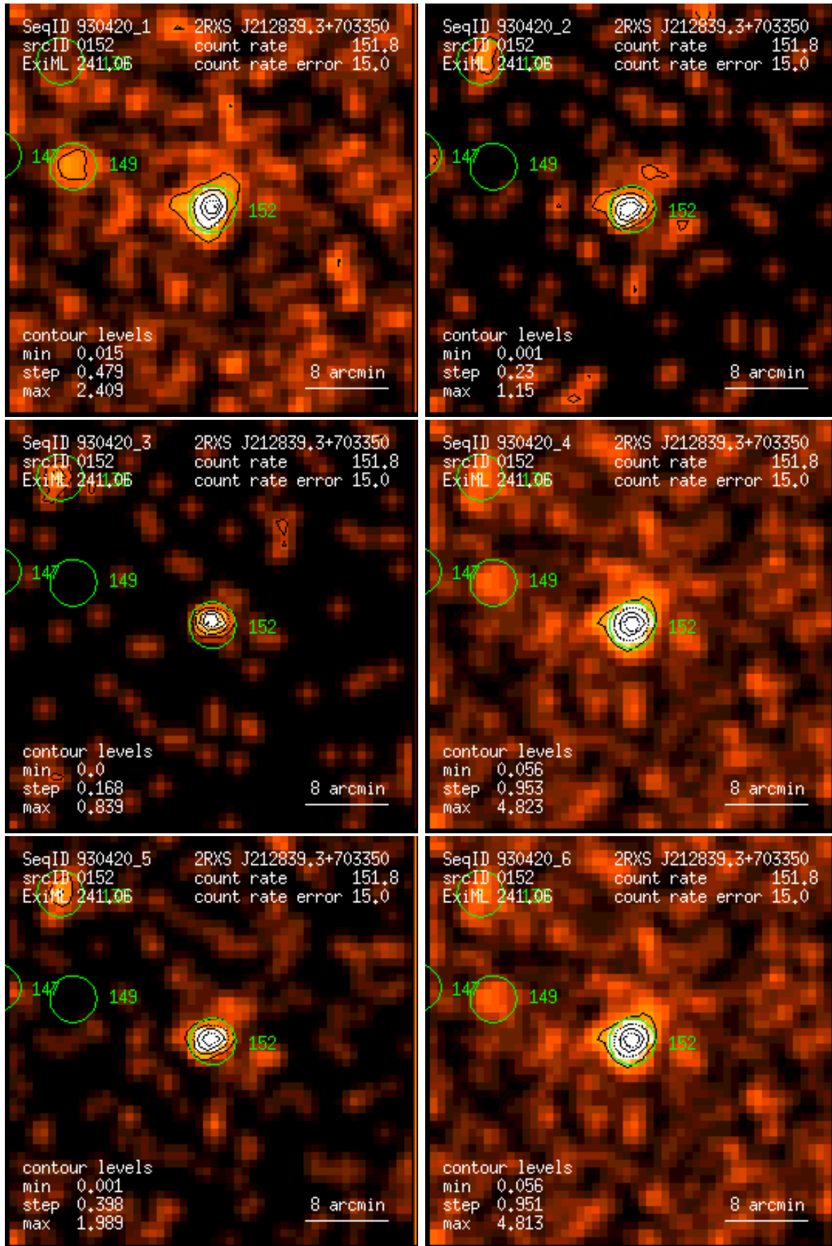
Figure 152: RASS 930420: detection 0152: band rate images, Gaussian filter: (1) PSPC channels 11 – 41, (2) 52 – 90, (3) 91 – 201, (4) 11 – 235, (5) 52 – 201, (6) 11 – 201. Broad band rates in counts/ks. Band rate contour levels in counts/ks/arcmin 2 .
