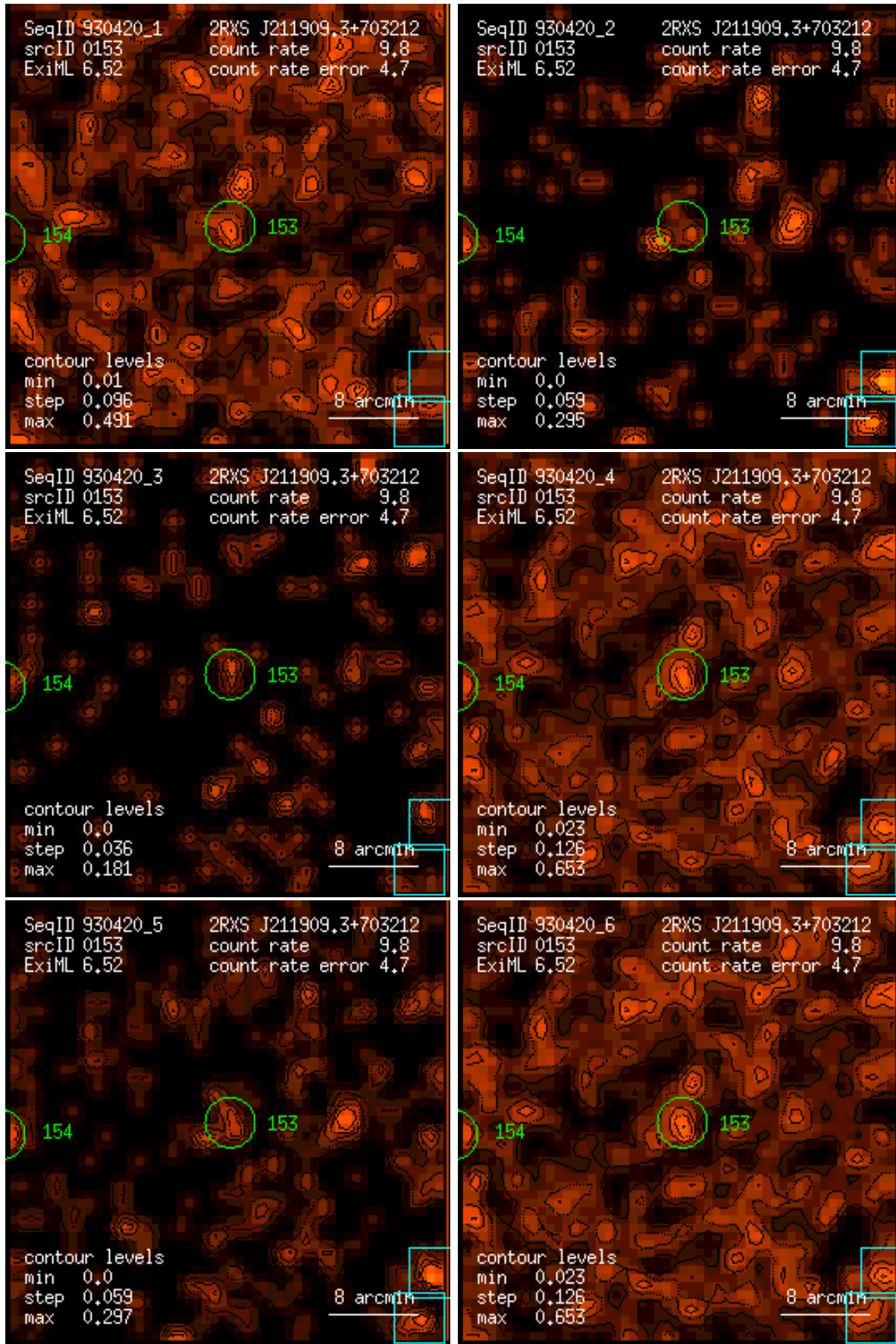
Figure 153: RASS 930420: detection 0153: band rate images, Gaussian filter: (1) PSPC channels 11 – 41, (2) 52 – 90, (3) 91 – 201, (4) 11 – 235, (5) 52 – 201, (6) 11 – 201. Broad band rates in counts/ks. Band rate contour levels in counts/ks/arcmin 2 .
