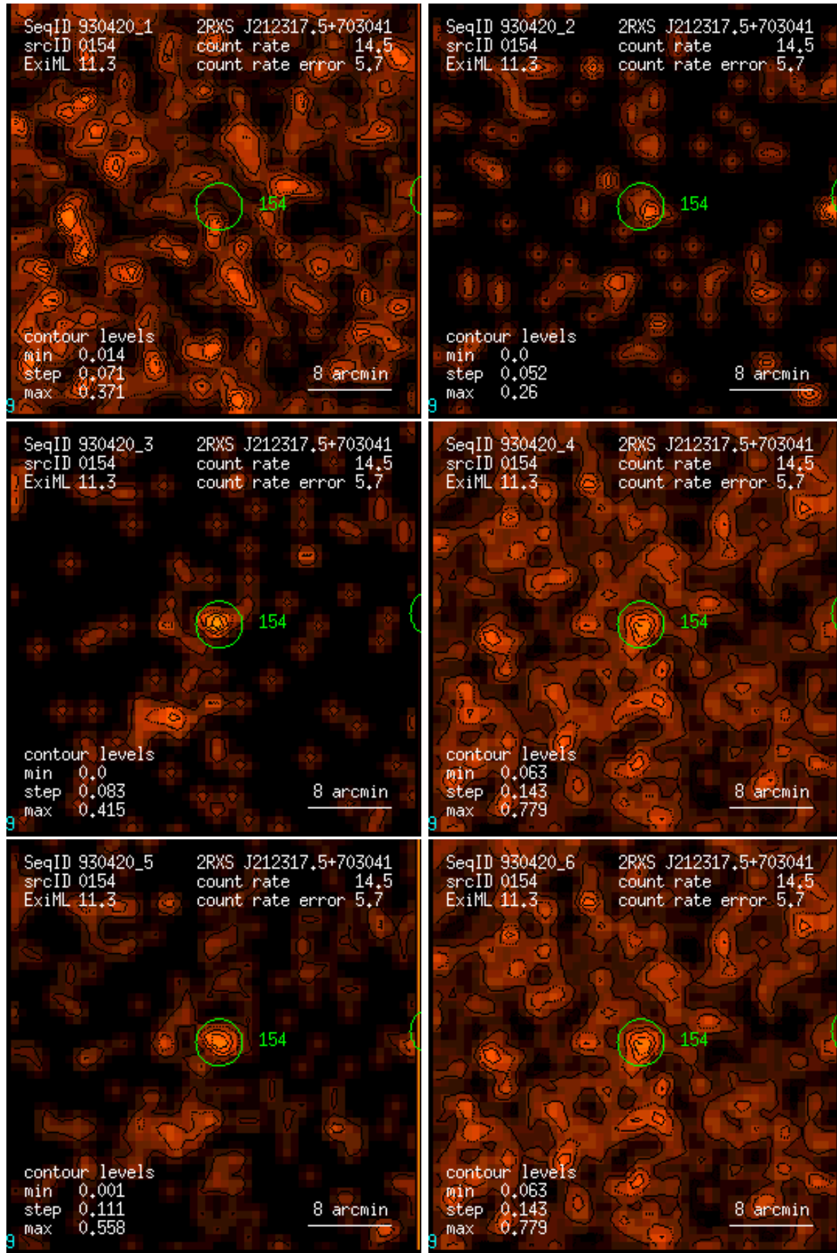
Figure 154: RASS 930420: detection 0154: band rate images, Gaussian filter: (1) PSPC channels 11 – 41, (2) 52 – 90, (3) 91 – 201, (4) 11 – 235, (5) 52 – 201, (6) 11 – 201. Broad band rates in counts/ks. Band rate contour levels in counts/ks/arcmin 2 .
