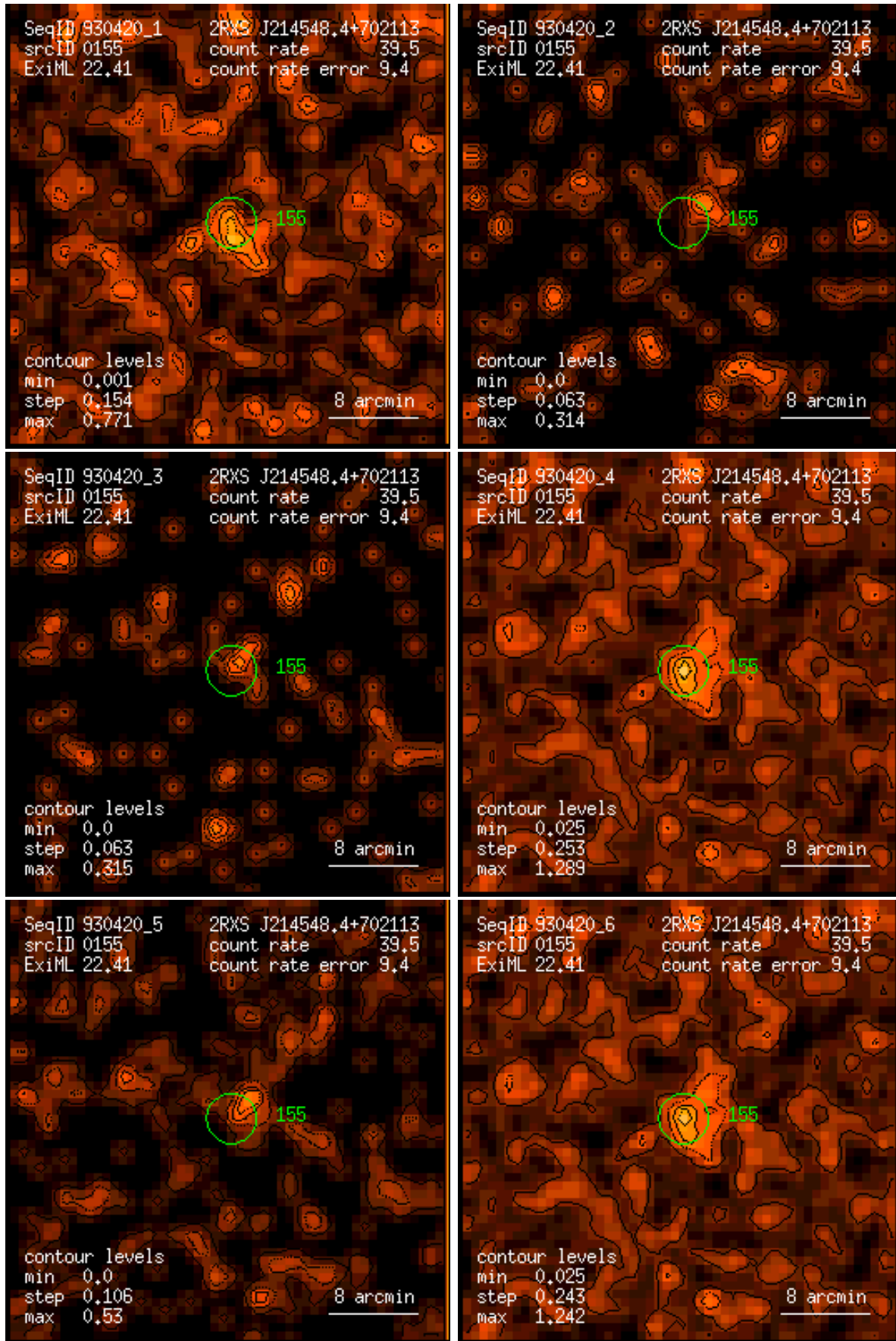
Figure 155: RASS 930420: detection 0155: band rate images, Gaussian filter: (1) PSPC channels 11 – 41, (2) 52 – 90, (3) 91 – 201, (4) 11 – 235, (5) 52 – 201, (6) 11 – 201. Broad band rates in counts/ks. Band rate contour levels in counts/ks/arcmin 2 .
