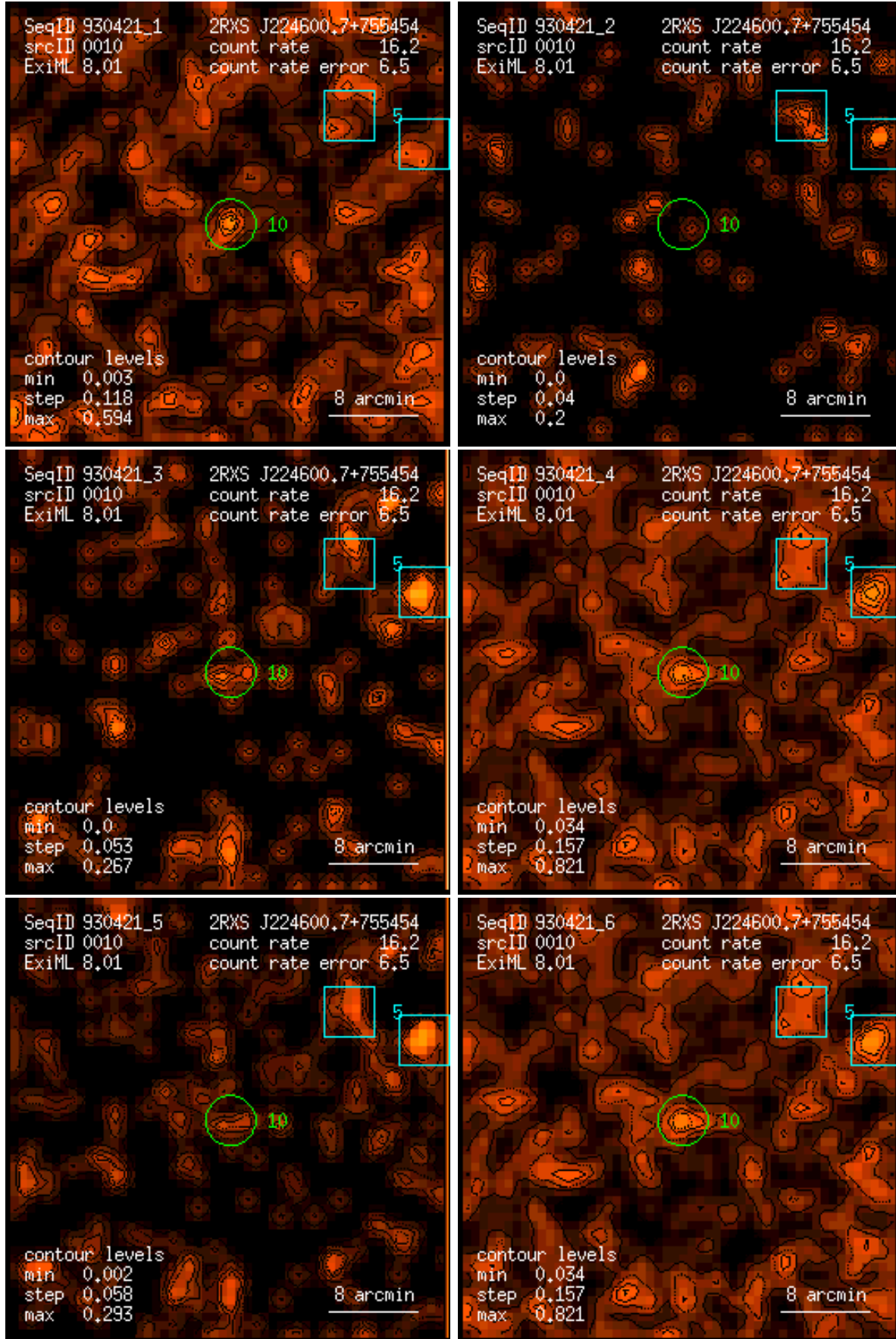
Figure 10: RASS 930421: detection 0010: band rate images, Gaussian filter: (1) PSPC channels 11 – 41, (2) 52 – 90, (3) 91 – 201, (4) 11 – 235, (5) 52 – 201, (6) 11 – 201. Broad band rates in counts/ks. Band rate contour levels in counts/ks/arcmin 2 .
