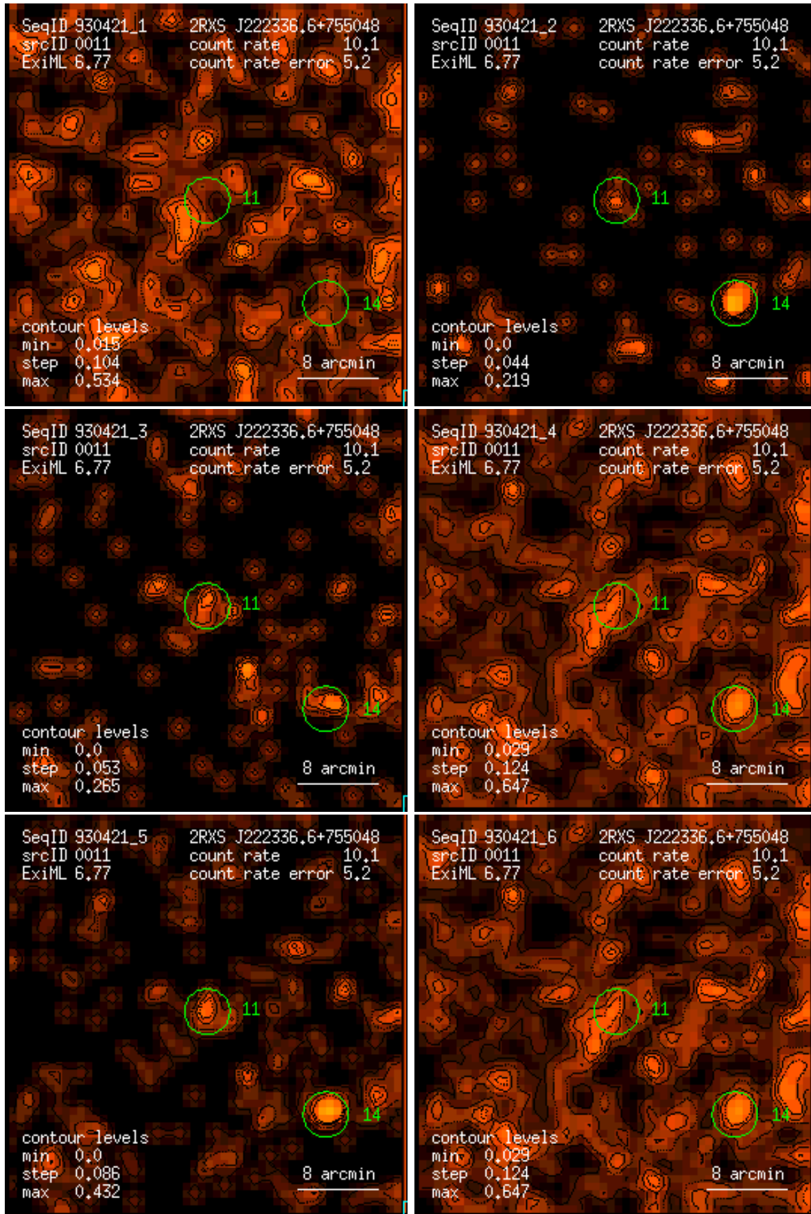
Figure 11: RASS 930421: detection 0011: band rate images, Gaussian filter: (1) PSPC channels 11 – 41, (2) 52 – 90, (3) 91 – 201, (4) 11 – 235, (5) 52 – 201, (6) 11 – 201. Broad band rates in counts/ks. Band rate contour levels in counts/ks/arcmin 2 .
