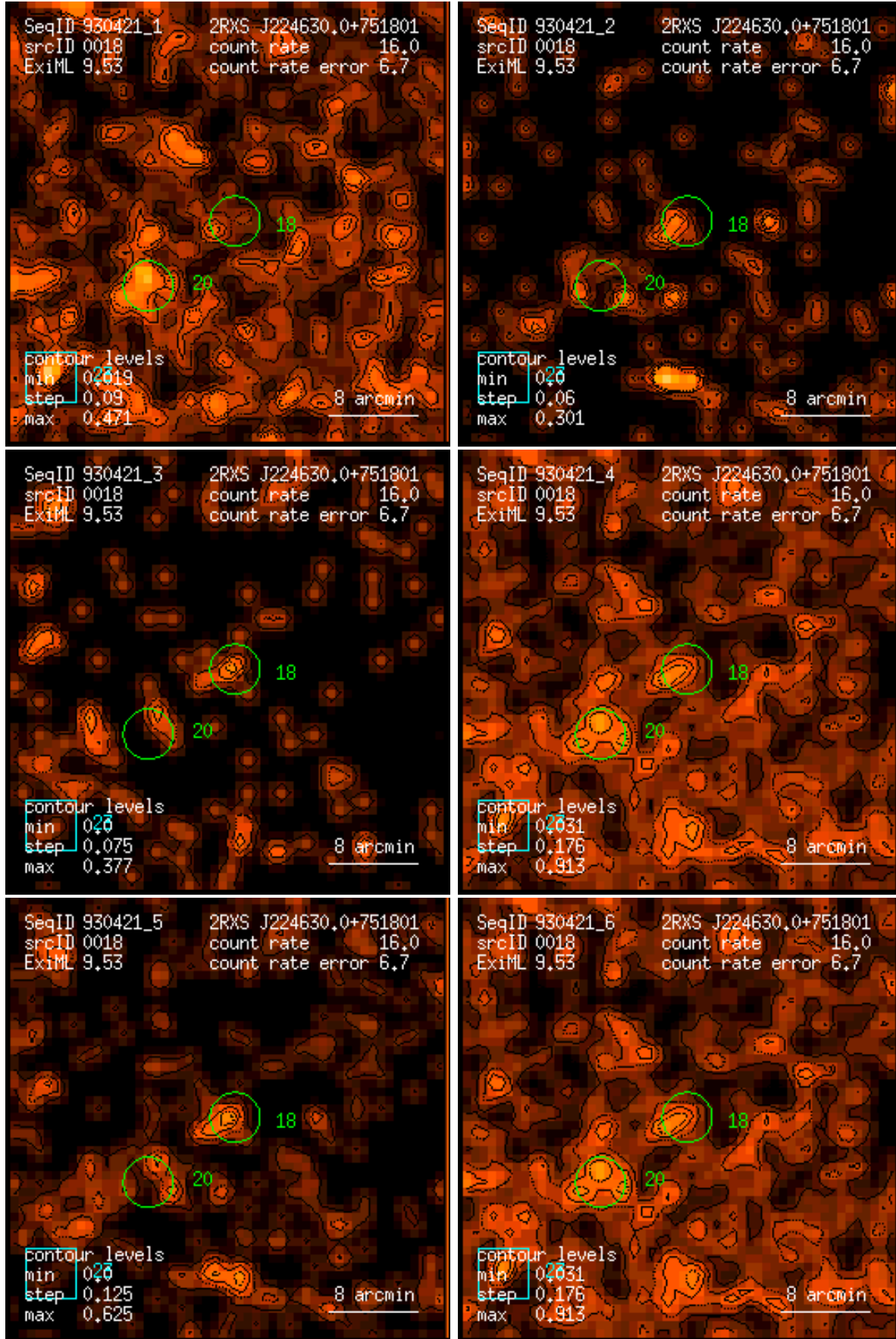
Figure 18: RASS 930421: detection 0018: band rate images, Gaussian filter: (1) PSPC channels 11 – 41, (2) 52 – 90, (3) 91 – 201, (4) 11 – 235, (5) 52 – 201, (6) 11 – 201. Broad band rates in counts/ks. Band rate contour levels in counts/ks/arcmin 2 .
