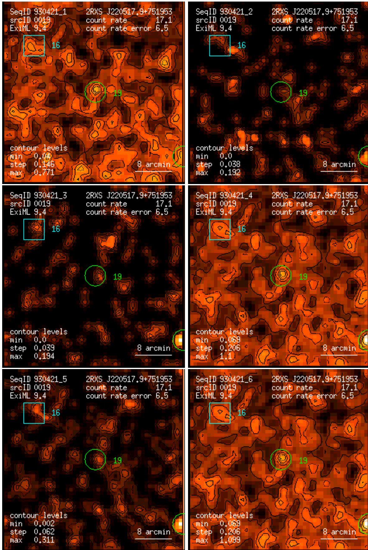
Figure 19: RASS 930421: detection 0019: band rate images, Gaussian filter: (1) PSPC channels 11 – 41, (2) 52 – 90, (3) 91 – 201, (4) 11 – 235, (5) 52 – 201, (6) 11 – 201. Broad band rates in counts/ks. Band rate contour levels in counts/ks/arcmin 2 .
