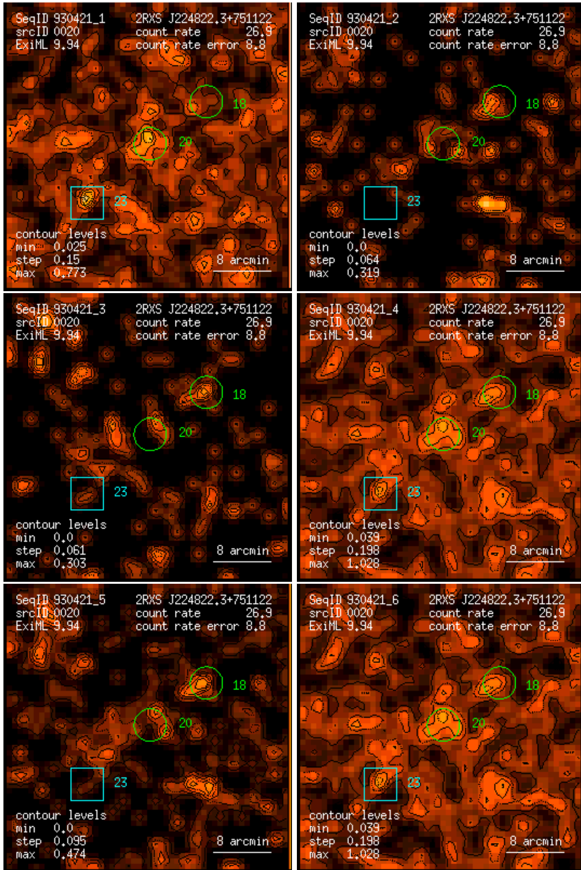
Figure 20: RASS 930421: detection 0020: band rate images, Gaussian filter: (1) PSPC channels 11 – 41, (2) 52 – 90, (3) 91 – 201, (4) 11 – 235, (5) 52 – 201, (6) 11 – 201. Broad band rates in counts/ks. Band rate contour levels in counts/ks/arcmin 2 .
