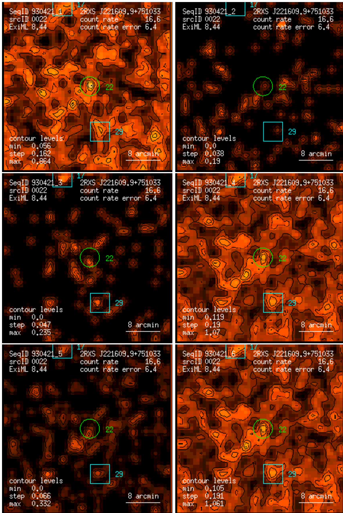
Figure 22: RASS 930421: detection 0022: band rate images, Gaussian filter: (1) PSPC channels 11 – 41, (2) 52 – 90, (3) 91 – 201, (4) 11 – 235, (5) 52 – 201, (6) 11 – 201. Broad band rates in counts/ks. Band rate contour levels in counts/ks/arcmin 2 .
