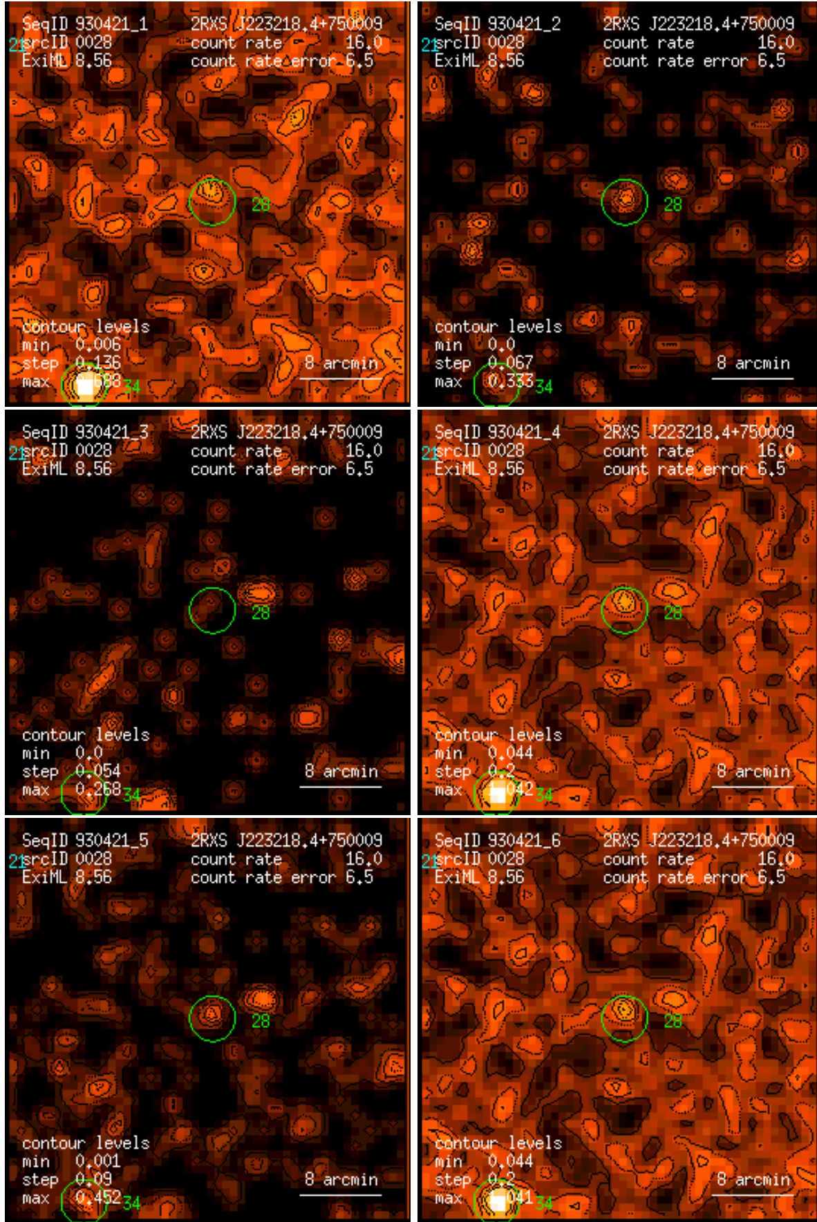
Figure 28: RASS 930421: detection 0028: band rate images, Gaussian filter: (1) PSPC channels 11 – 41, (2) 52 – 90, (3) 91 – 201, (4) 11 – 235, (5) 52 – 201, (6) 11 – 201. Broad band rates in counts/ks. Band rate contour levels in counts/ks/arcmin 2 .
