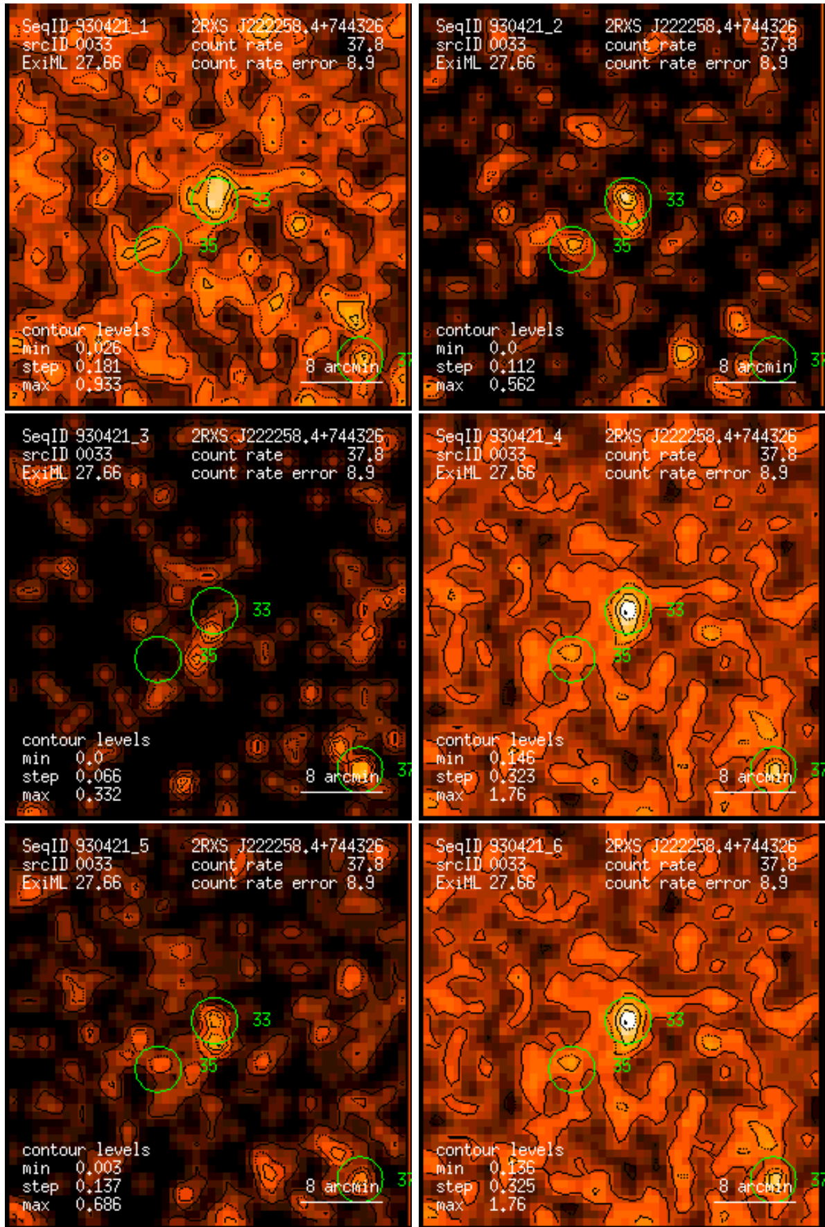
Figure 33: RASS 930421: detection 0033: band rate images, Gaussian filter: (1) PSPC channels 11 – 41, (2) 52 – 90, (3) 91 – 201, (4) 11 – 235, (5) 52 – 201, (6) 11 – 201. Broad band rates in counts/ks. Band rate contour levels in counts/ks/arcmin 2 .
