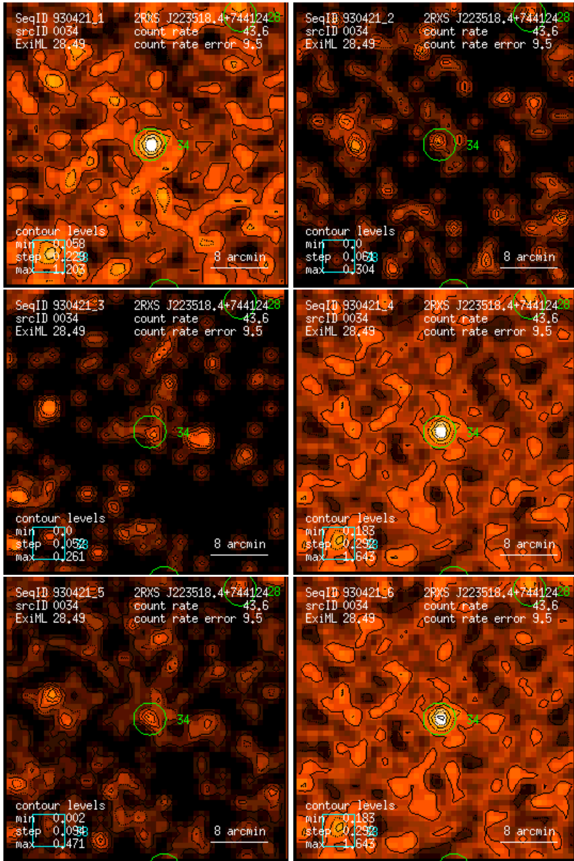
Figure 34: RASS 930421: detection 0034: band rate images, Gaussian filter: (1) PSPC channels 11 – 41, (2) 52 – 90, (3) 91 – 201, (4) 11 – 235, (5) 52 – 201, (6) 11 – 201. Broad band rates in counts/ks. Band rate contour levels in counts/ks/arcmin 2 .
