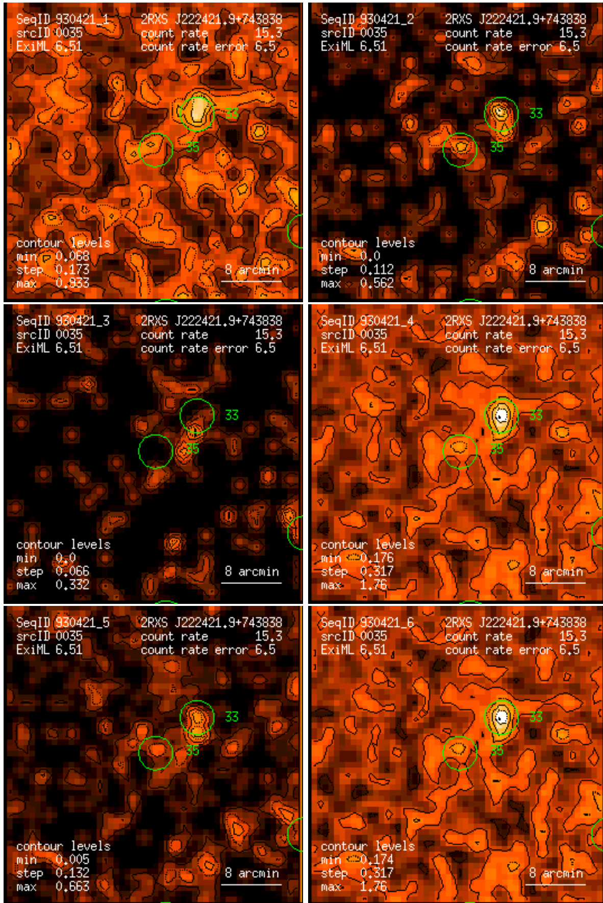
Figure 35: RASS 930421: detection 0035: band rate images, Gaussian filter: (1) PSPC channels 11 – 41, (2) 52 – 90, (3) 91 – 201, (4) 11 – 235, (5) 52 – 201, (6) 11 – 201. Broad band rates in counts/ks. Band rate contour levels in counts/ks/arcmin 2 .
