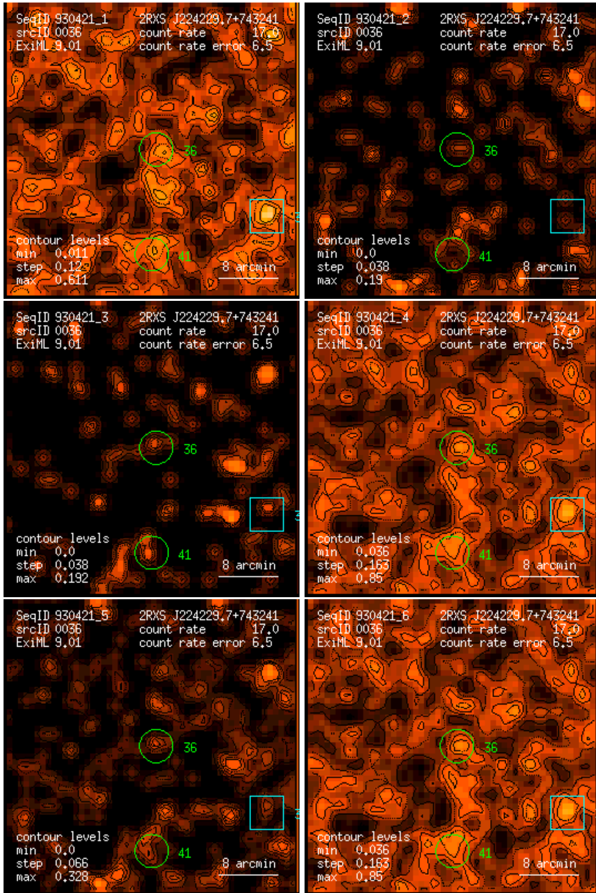
Figure 36: RASS 930421: detection 0036: band rate images, Gaussian filter: (1) PSPC channels 11 – 41, (2) 52 – 90, (3) 91 – 201, (4) 11 – 235, (5) 52 – 201, (6) 11 – 201. Broad band rates in counts/ks. Band rate contour levels in counts/ks/arcmin 2 .
